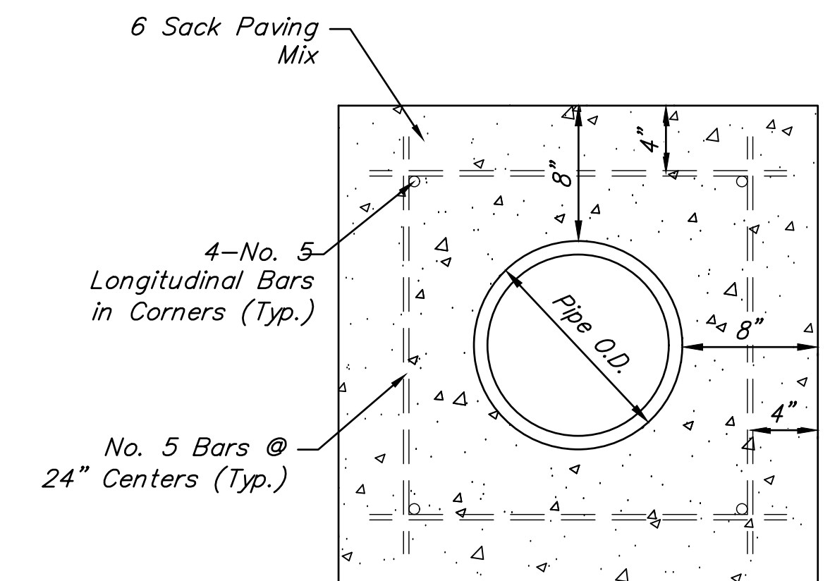
CONCRETE ENCASEMENT DETAIL
