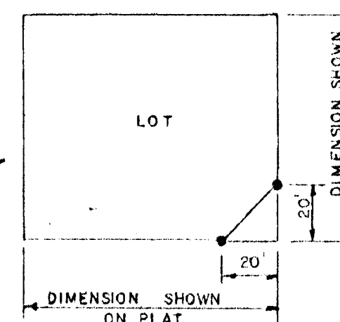
TYPICAL INTERSECTION RIGHT OF WAY DETAILS
