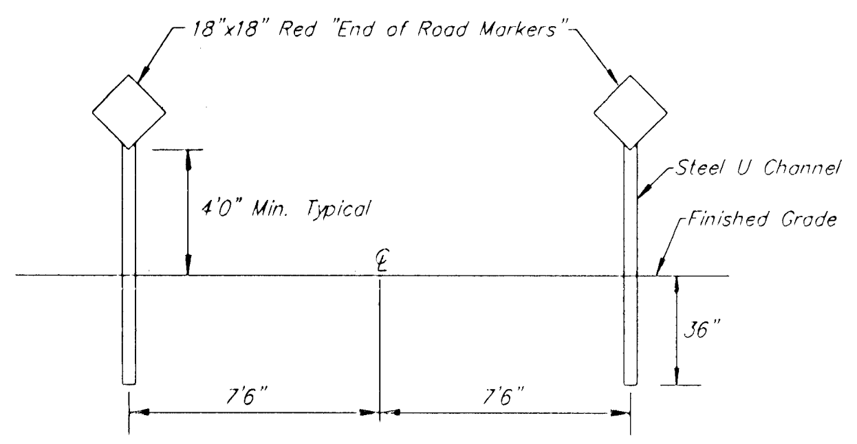
Barricade Detail
