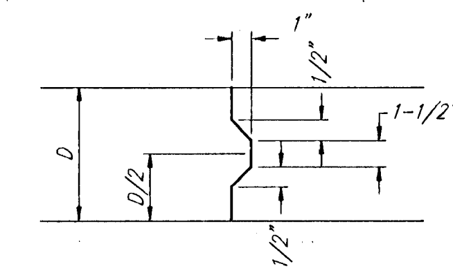
KEYWAY DETAIL
