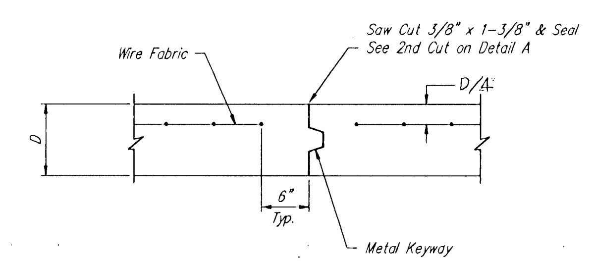
OPTIONAL CONTRACTION CONST. JOINT (C.J.) (ALTERNATE C.J.)
