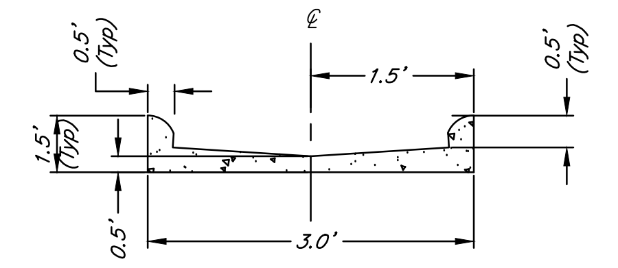
Typical Flume Section
