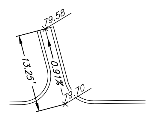
Typical Flume Plan
