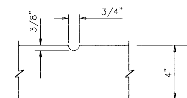
GROOVE DETAIL
