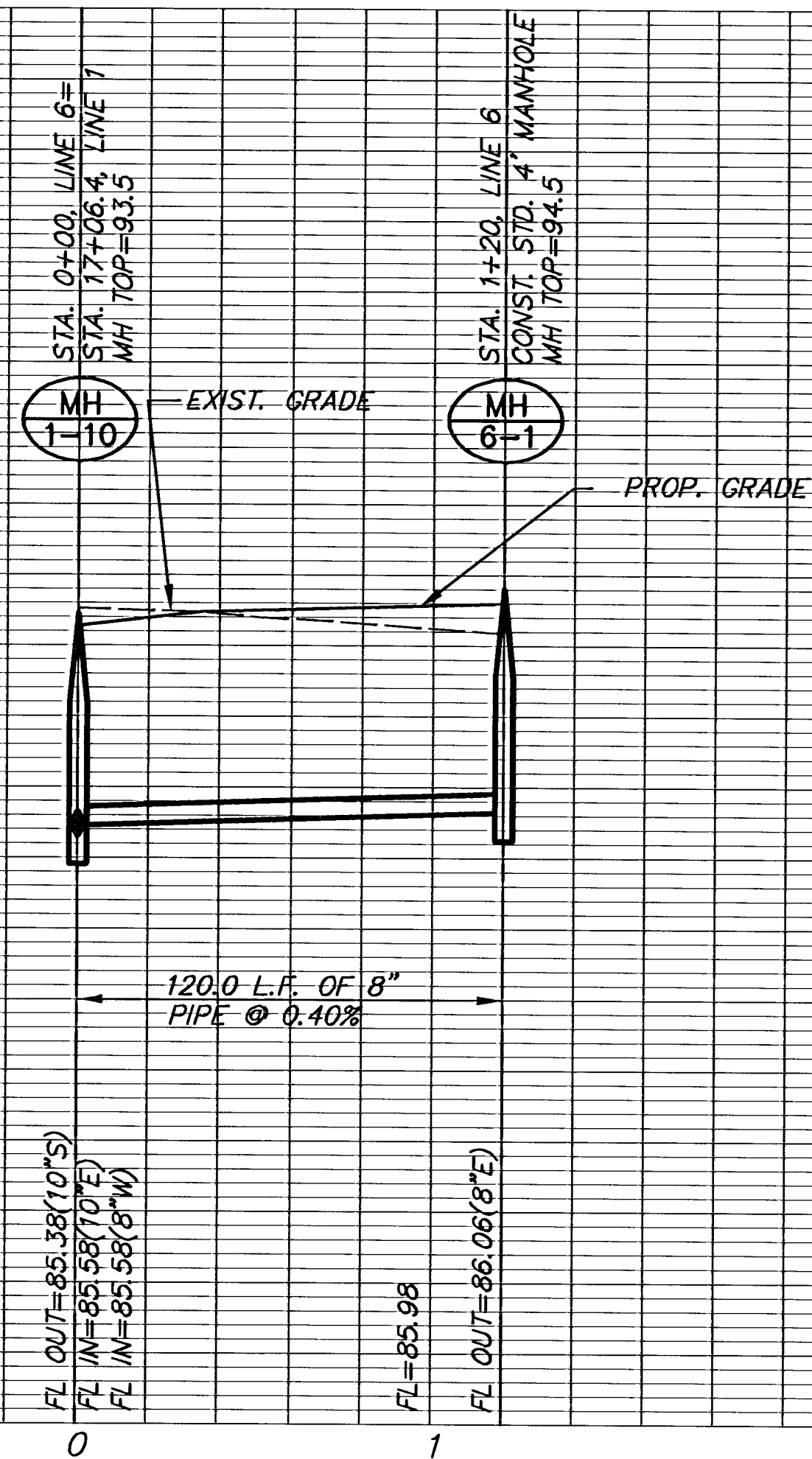
PROFILE LINE 6
