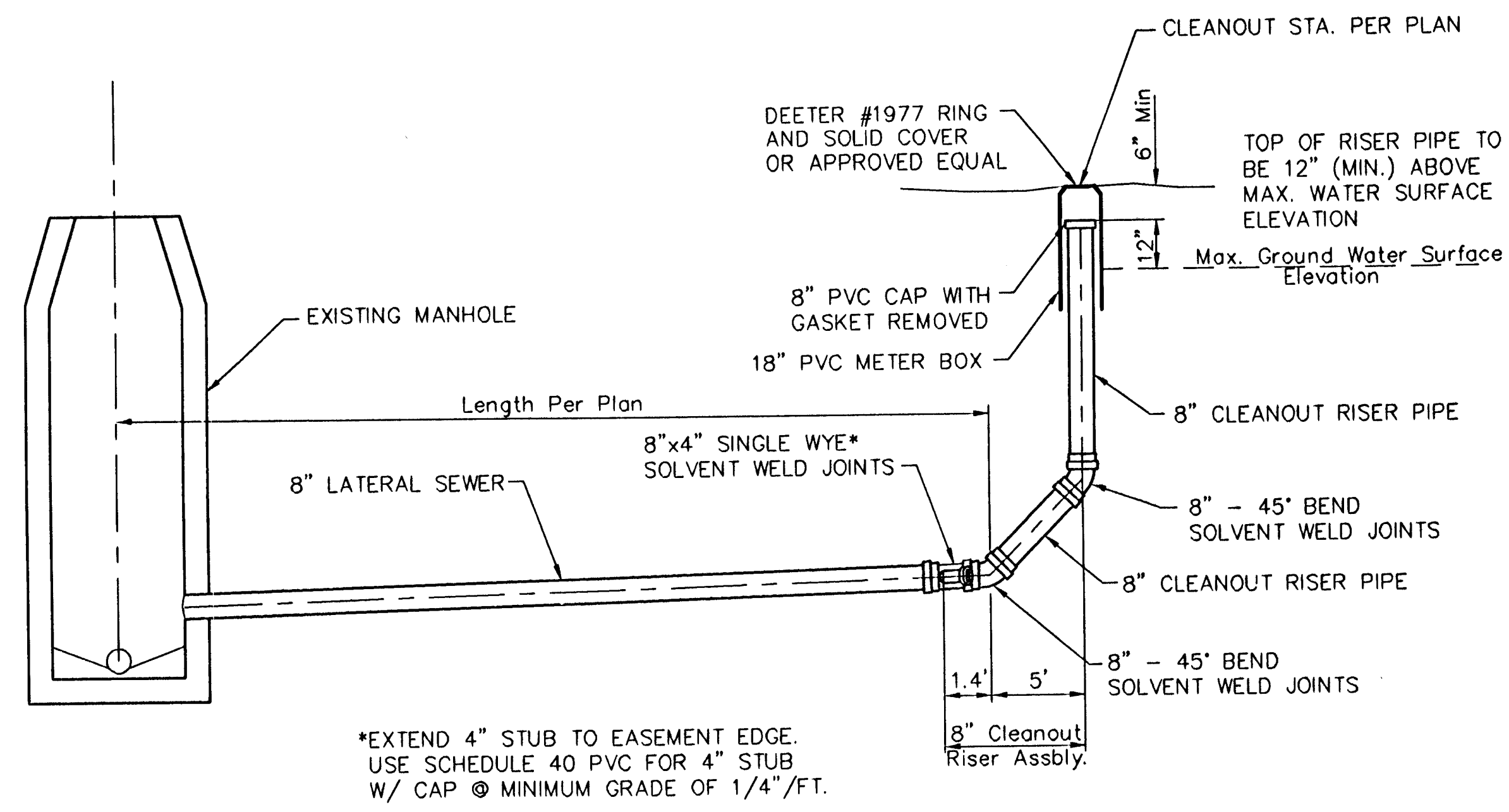
8" CLEANOUT RISER ASSEMBLY DETAIL
