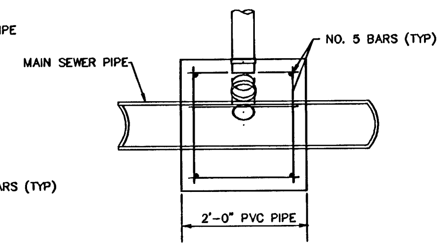
SECTION X-X
