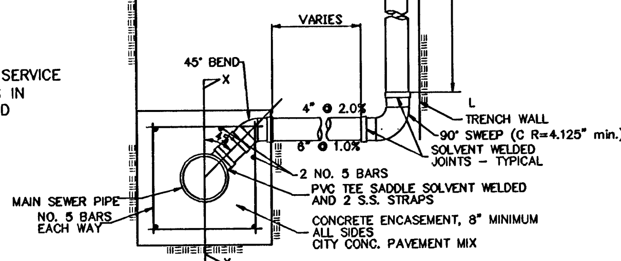
TYPICAL RISER DETAIL
