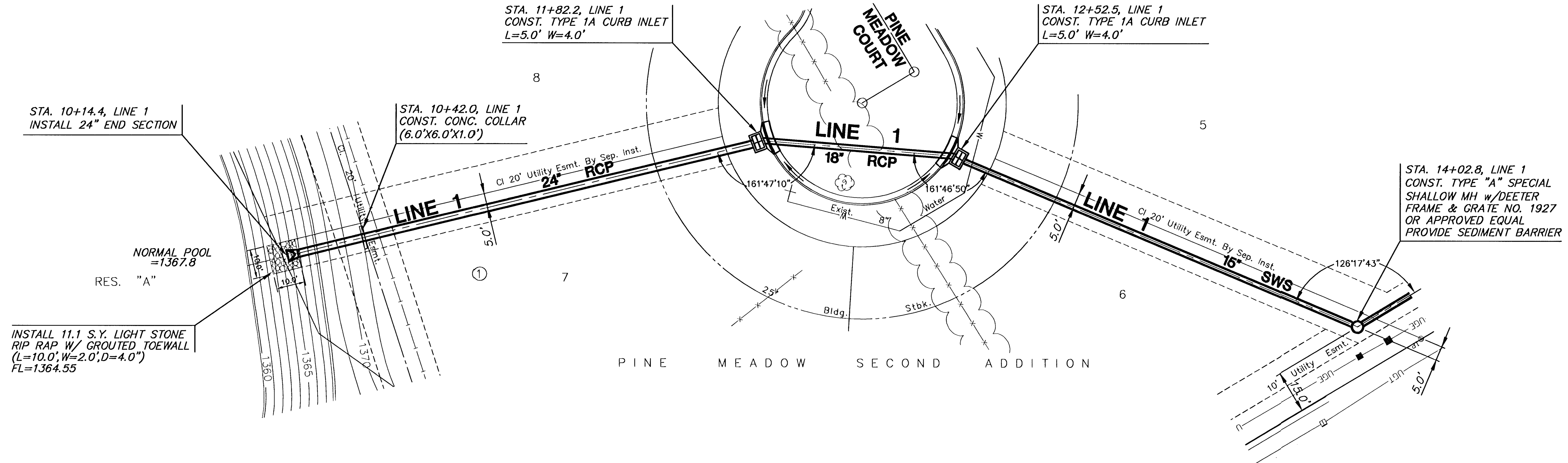
PLAN LINE 1
