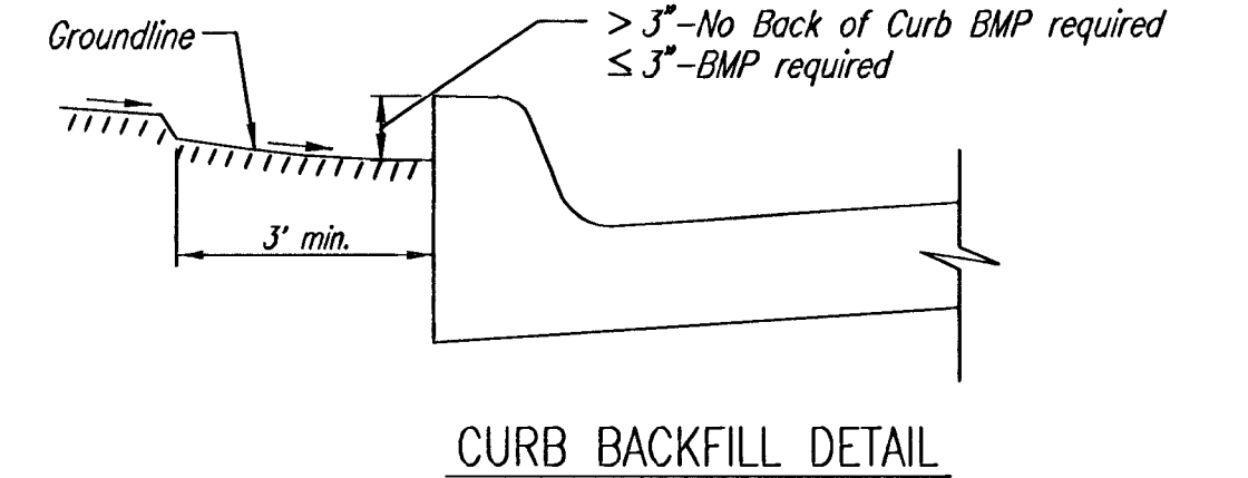
CURB BACKFILL DETAIL
