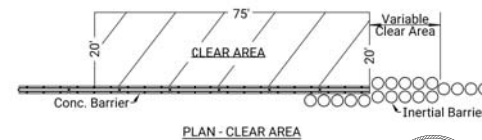
PLAN - CLEAR AREA
