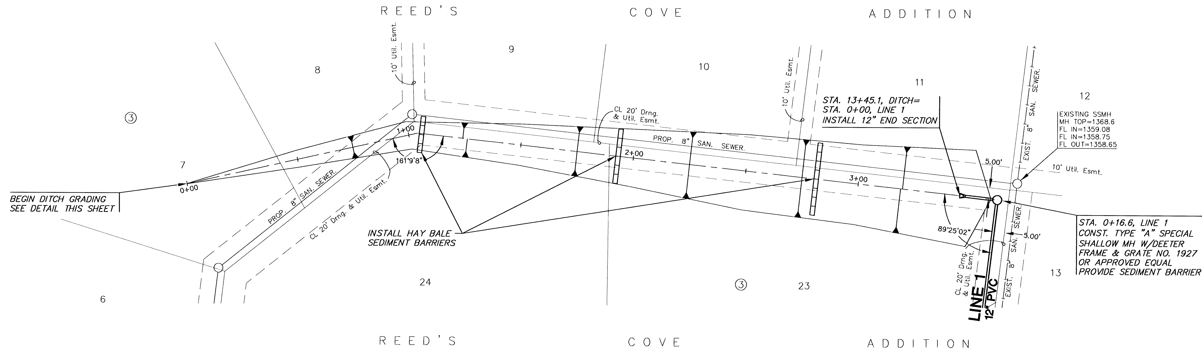
PLAN DITCH
