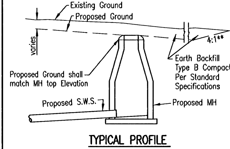
TYPICAL PROFILE
