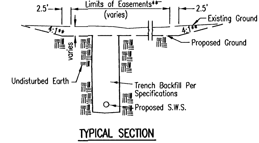
TYPICAL SECTION
