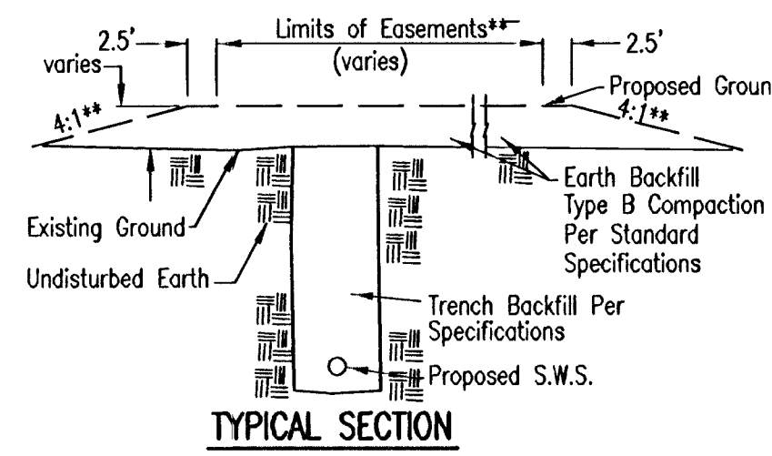
TYPICAL SECTION
