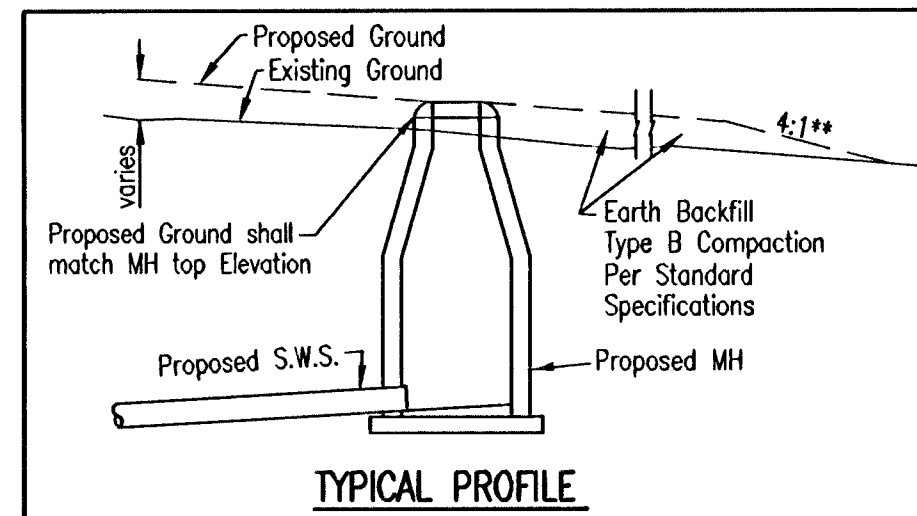
TYPICAL PROFILE
