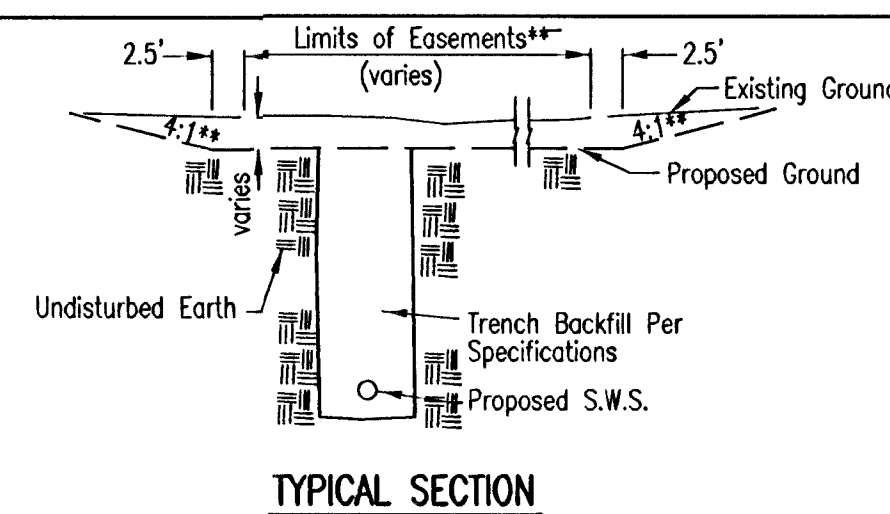
TYPICAL SECTION
