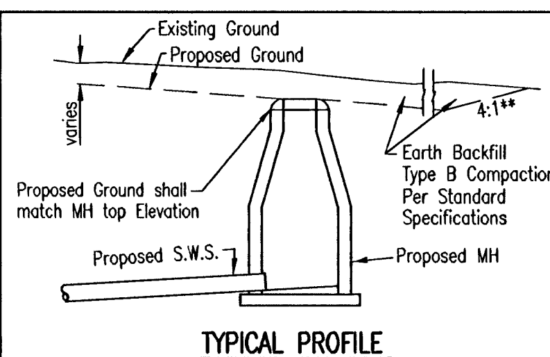
TYPICAL PROFILE
