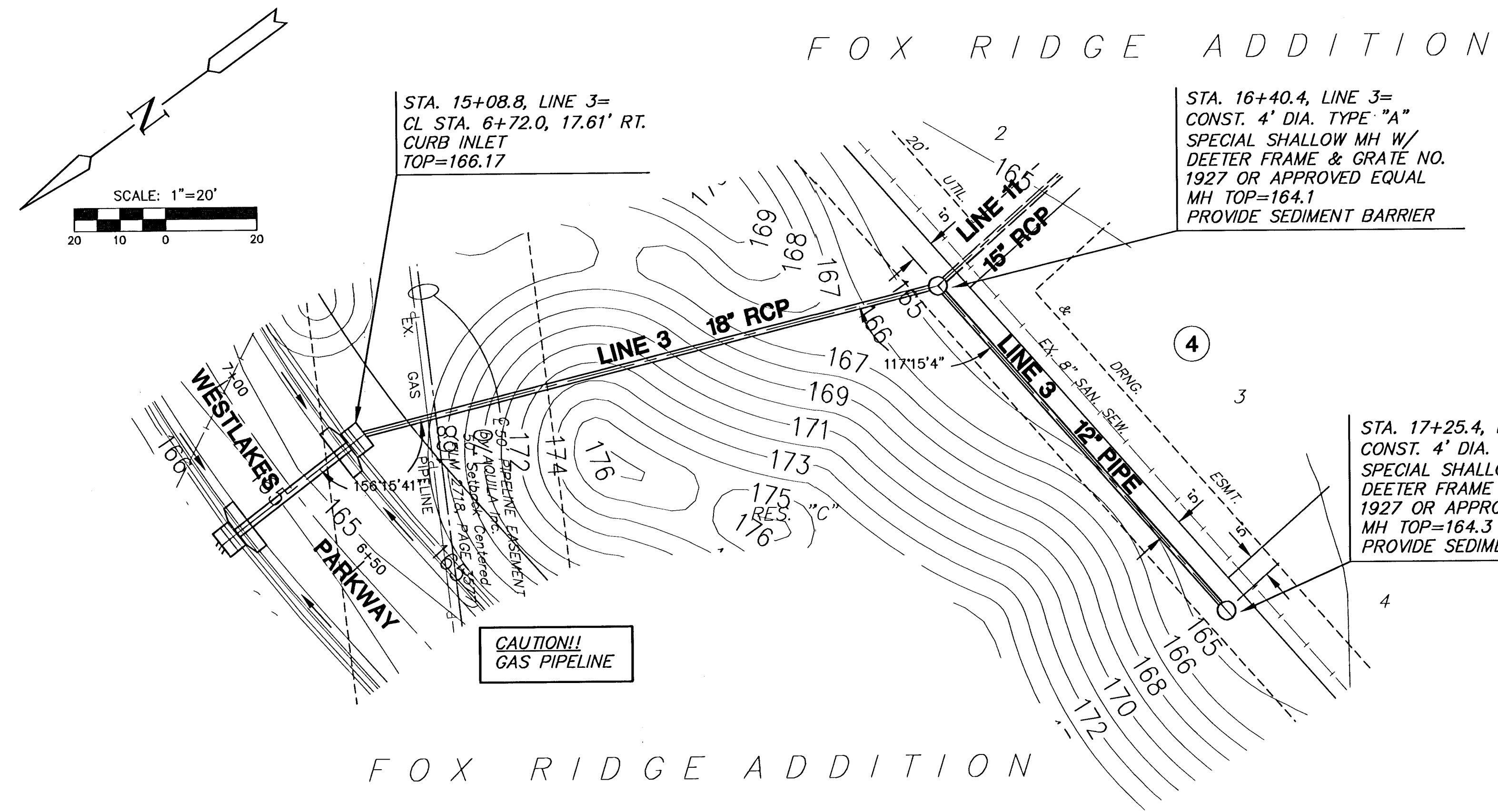
PLAN LINE 3
