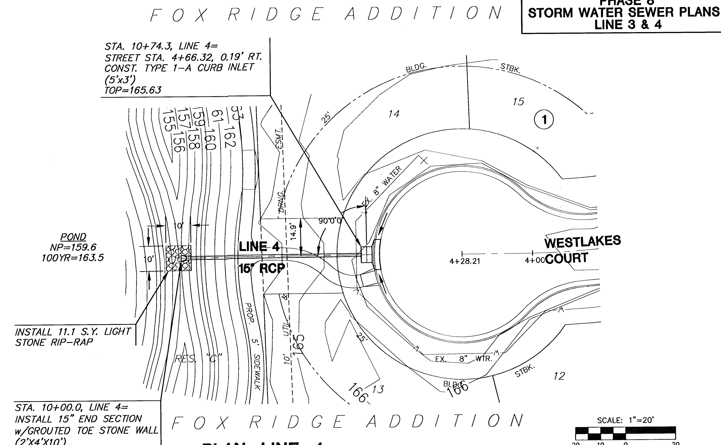
PLAN LINE 4
