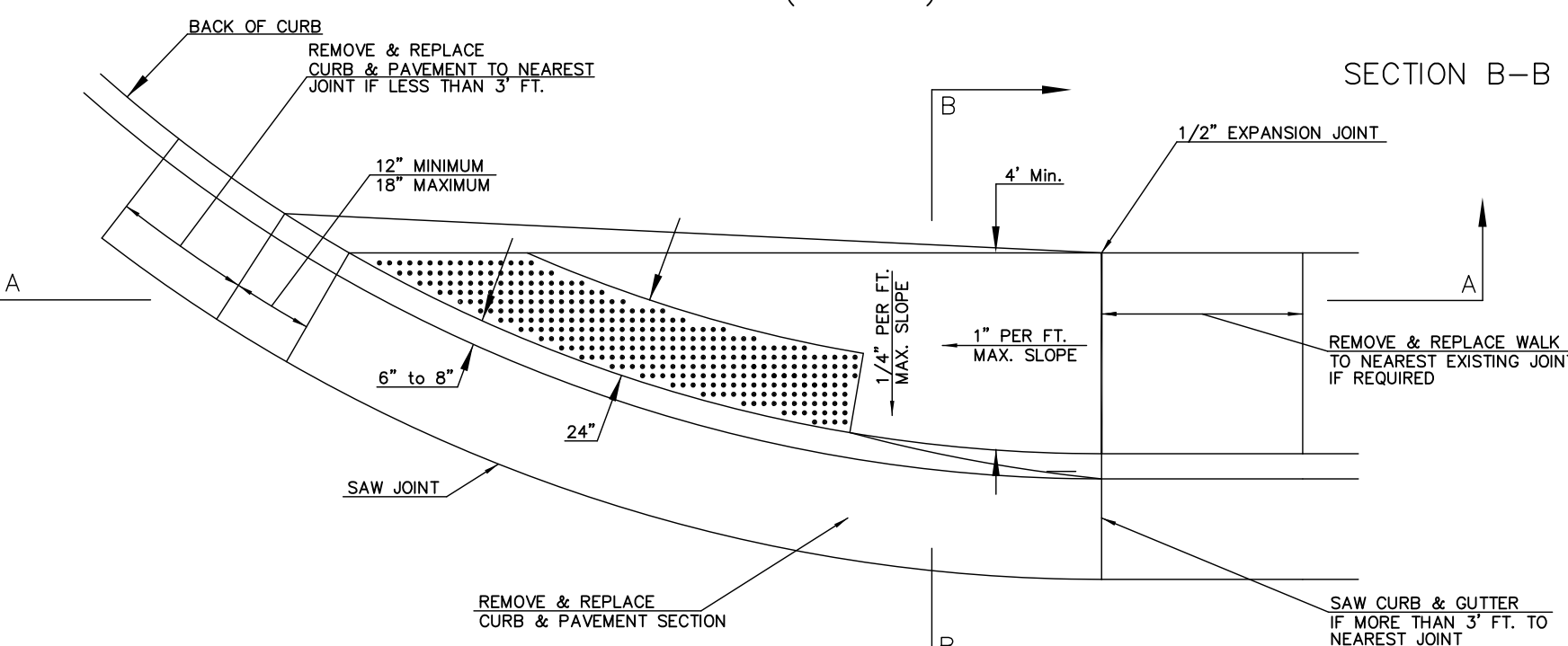
SECTION B-B
