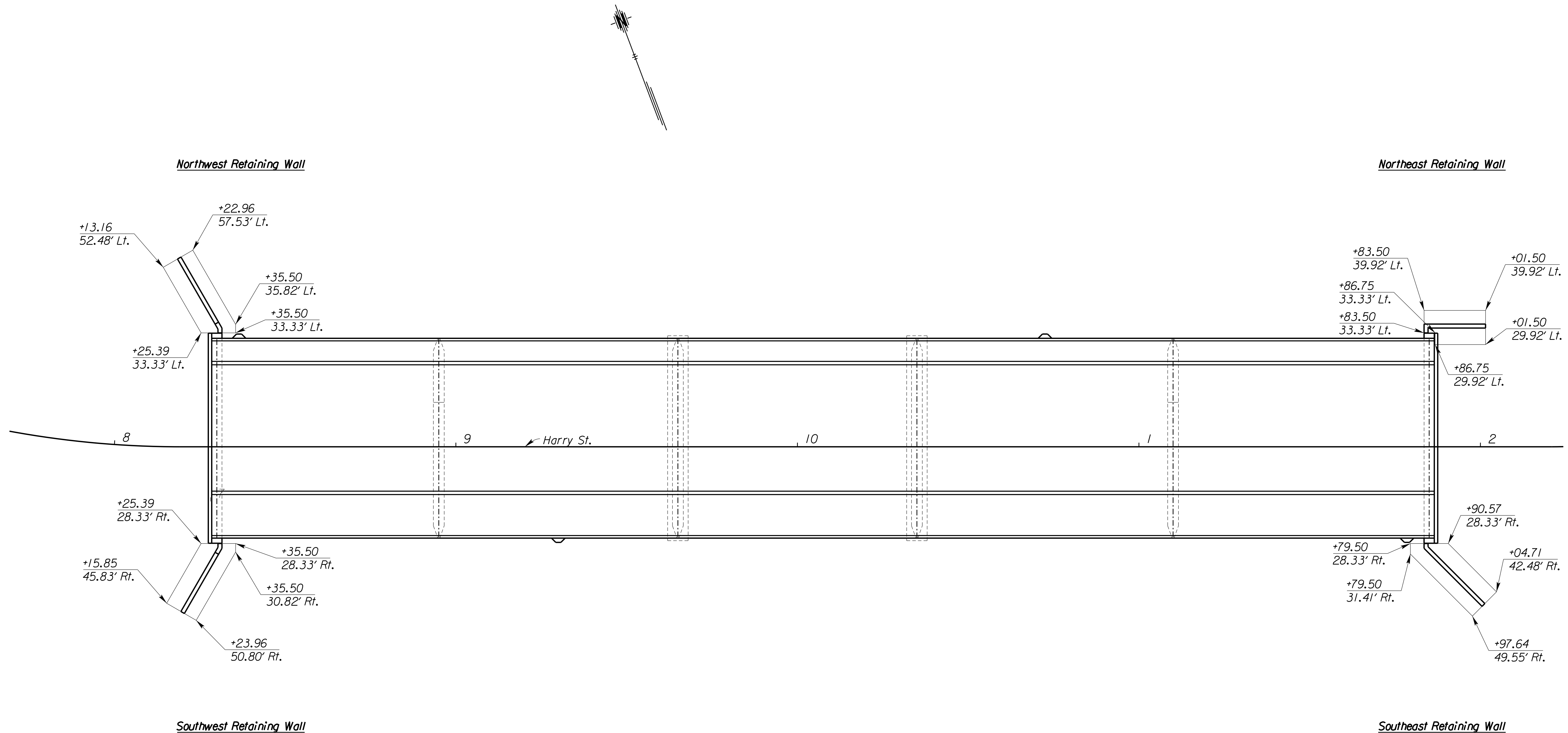
PLAN Providing Station/Offsets for corners of Retaining Wall Footings. Station/Offsets from @ Harry St.
