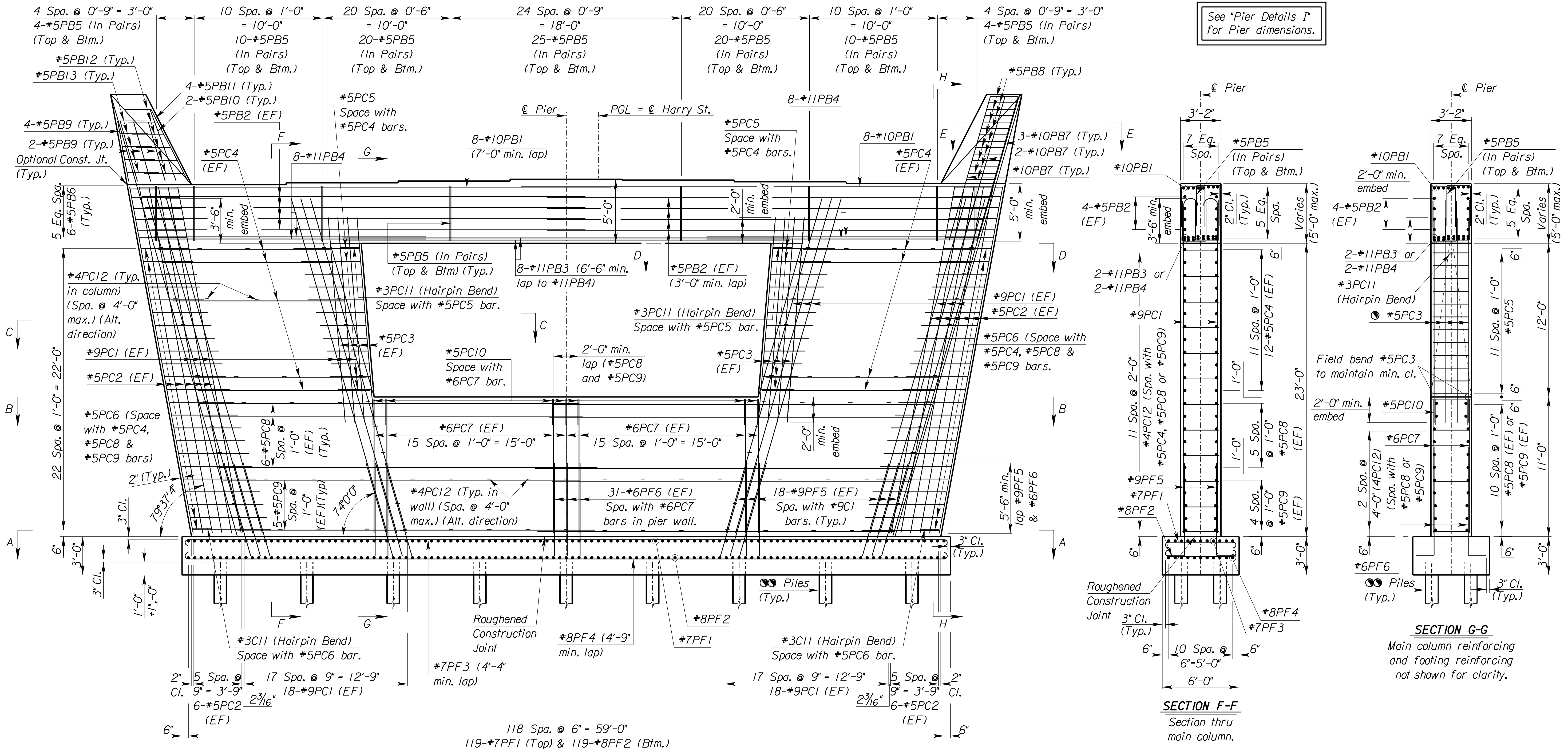
ELEVATION Piers 2 & 3 shown. (Piers 1 & 4 similar above footing)
