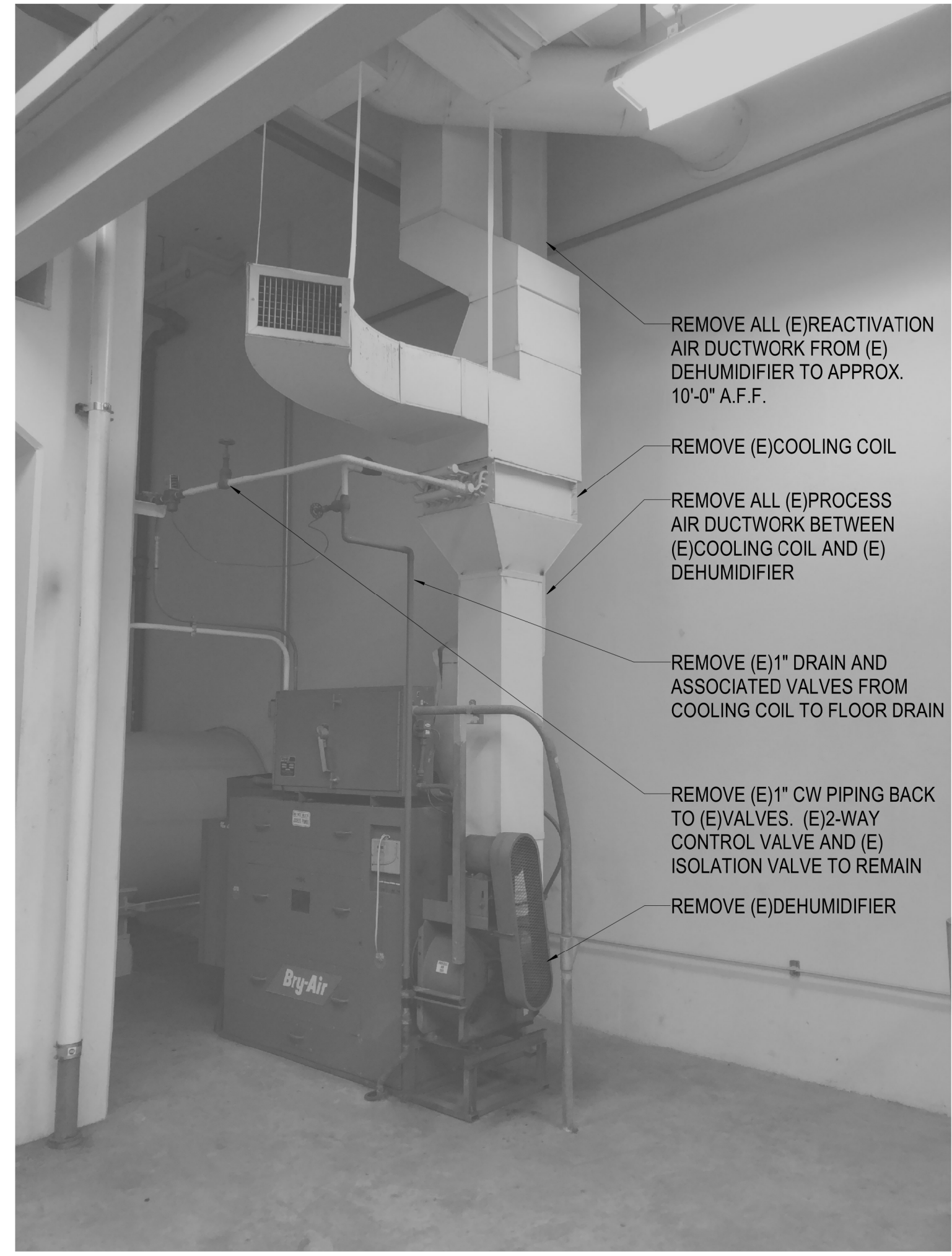
4 DEHUMIDIFIER 4 DEMO NO SCALE BASE BID
