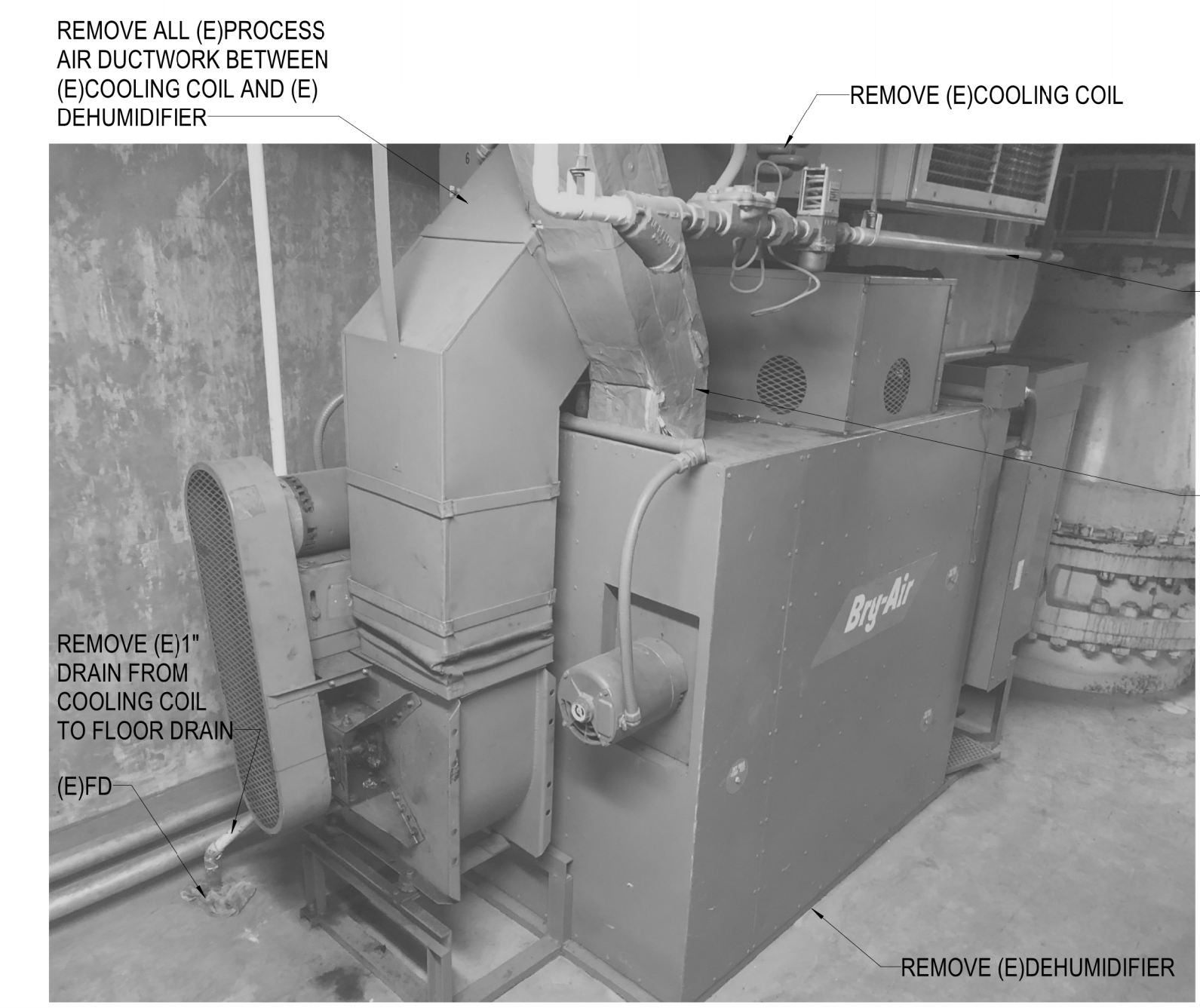
6 DEHUMIDIFIER 6 DEMO NO SCALE ALT. 2
