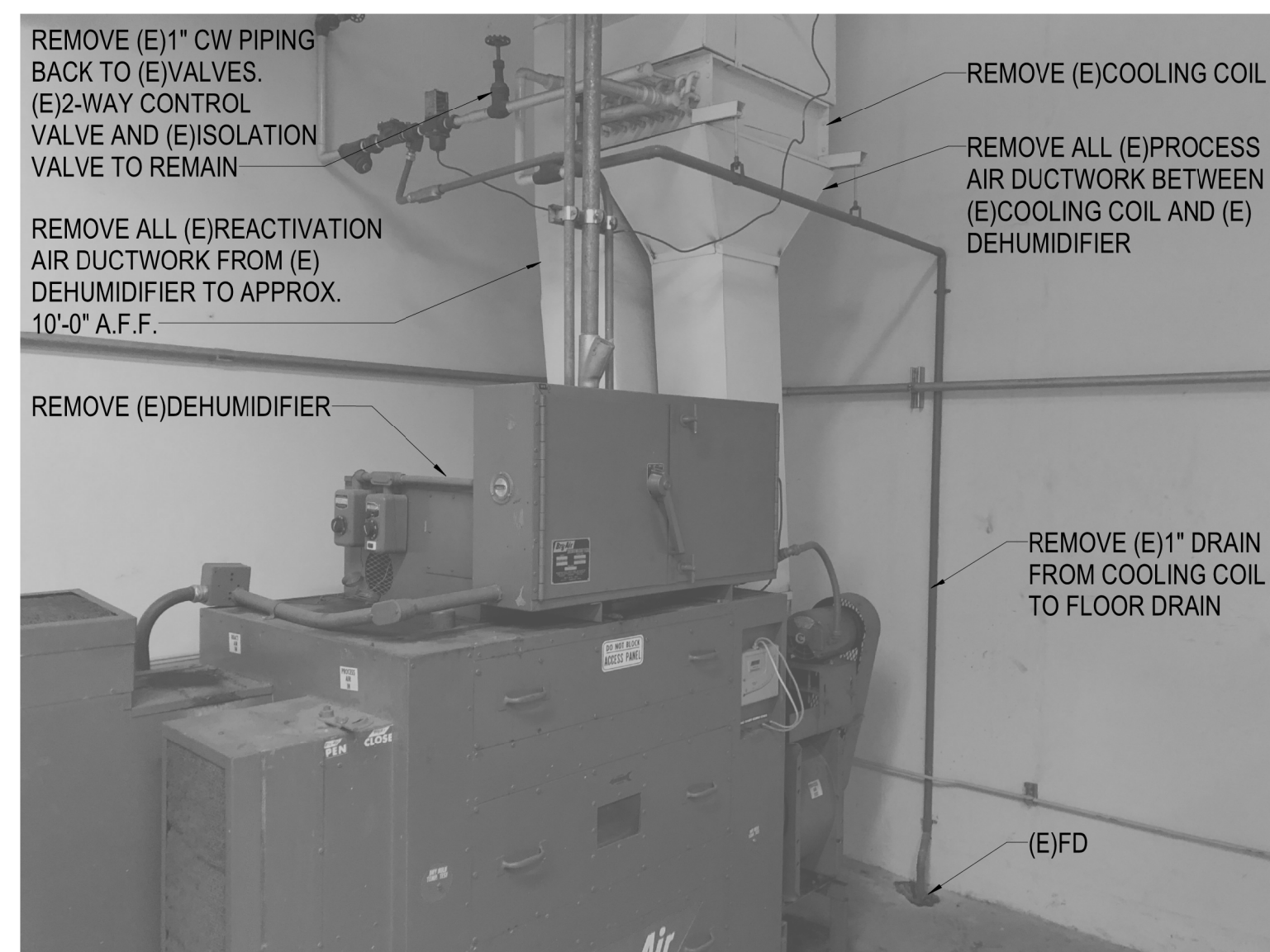
1 DEHUMIDIFIER 1 DEMO NO SCALE BASE BID
