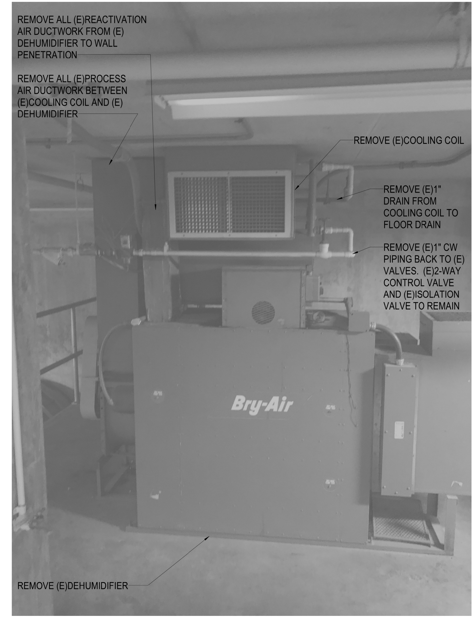
5 DEHUMIDIFIER 5 DEMO NO SCALE ALT. 1
