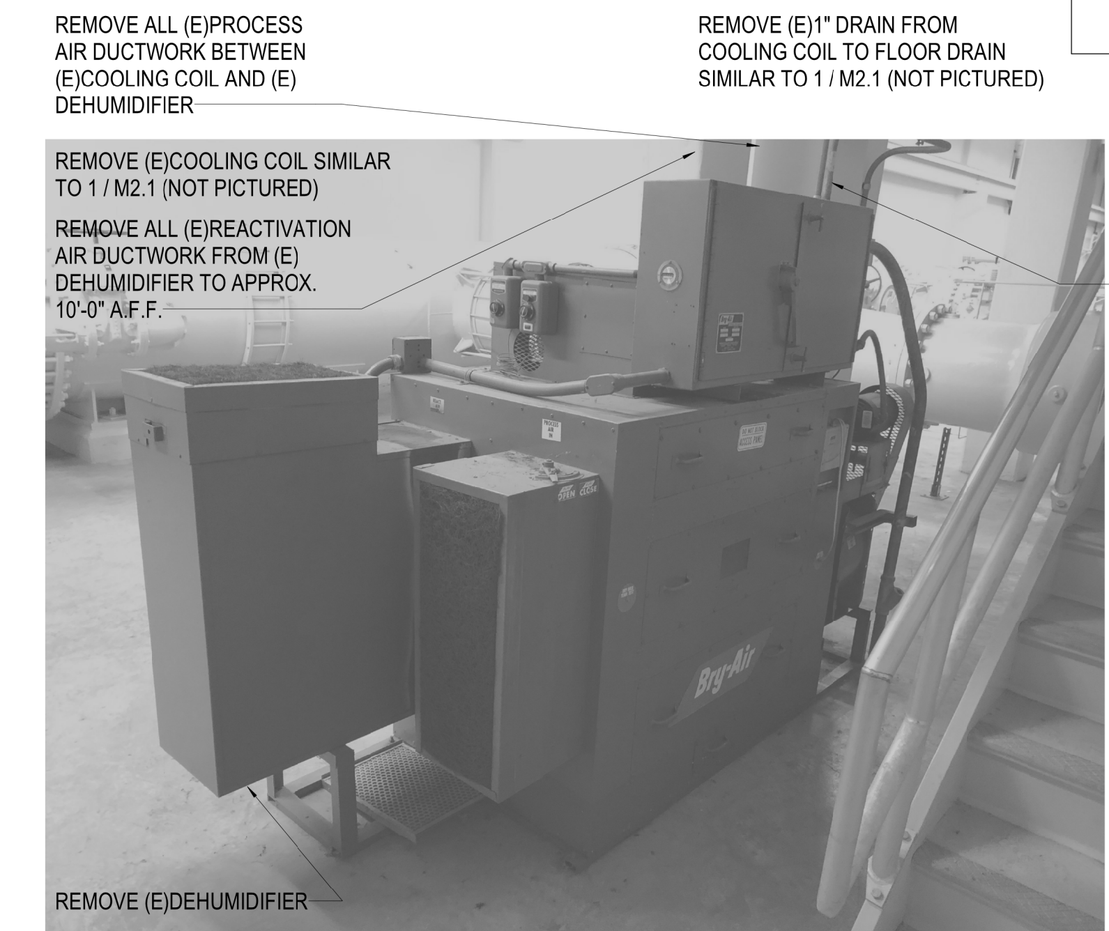
3 DEHUMIDIFIER 3 DEMO NO SCALE BASE BID
