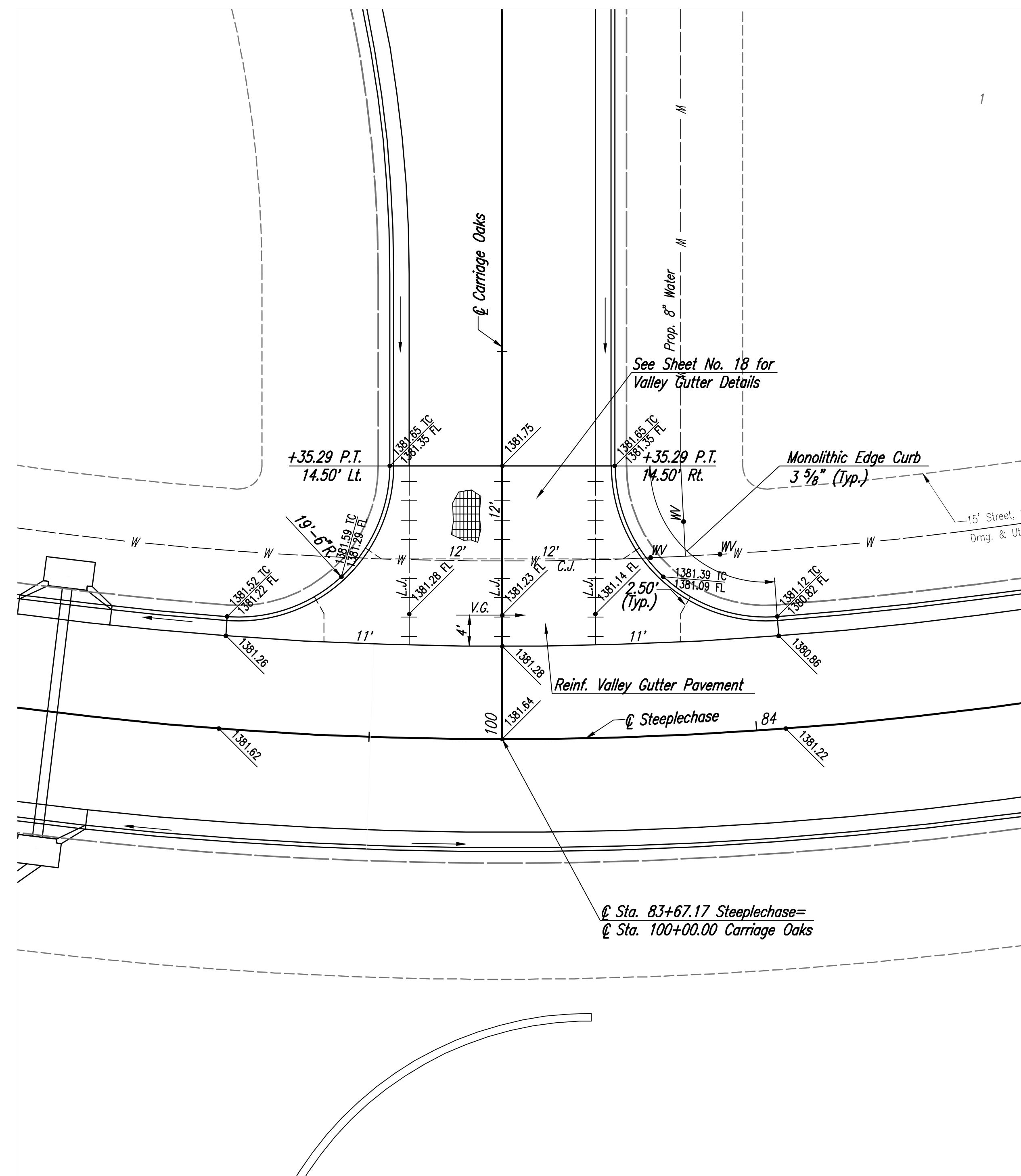
VALLEY GUTTER
