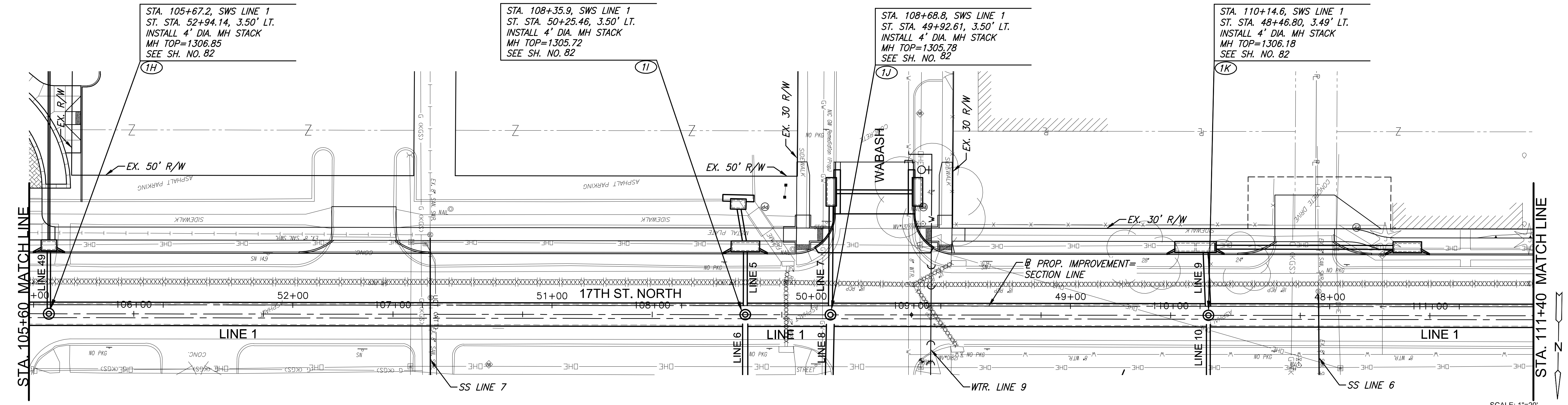
PLAN LINE 1 (CONT. 1) PROFILE LINE 1 (CONT. 1)
