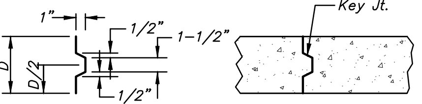
ALT. LONGITUDINAL CONSTRUCTION JOINT
