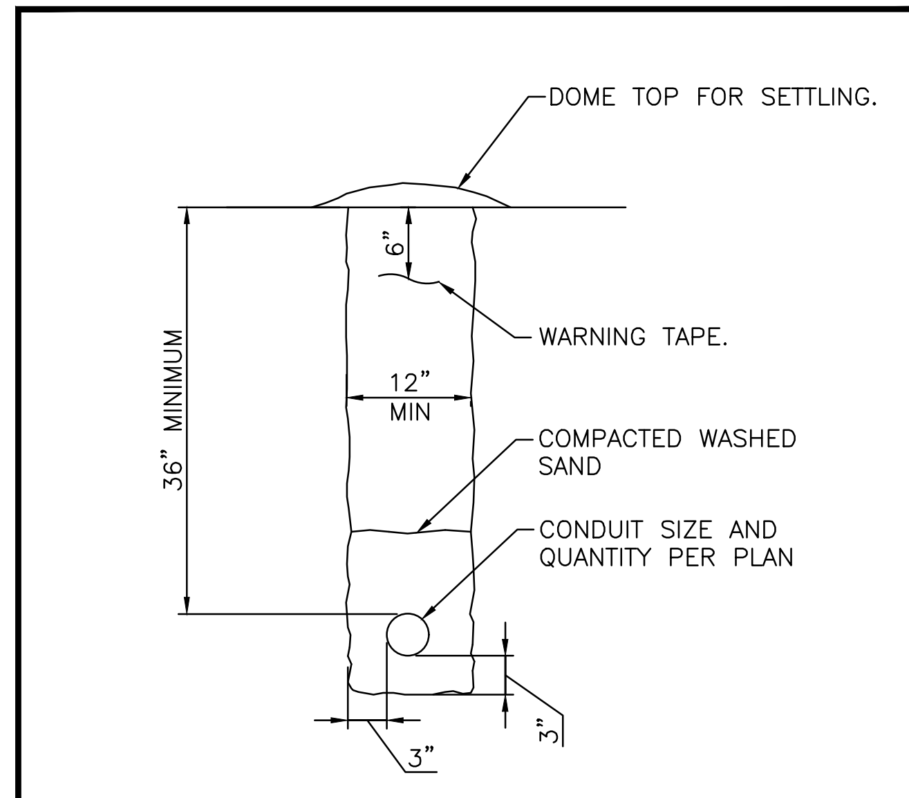
1 NO SCALE TYPICAL TRENCH CROSS SECTION
