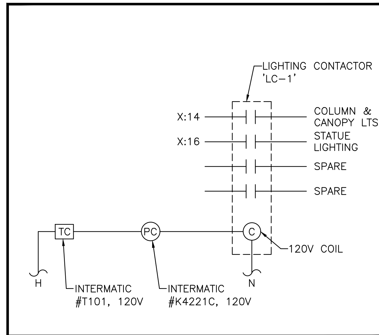
2 NO SCALE LIGHTING CONTACTOR CONTROL DETAIL
