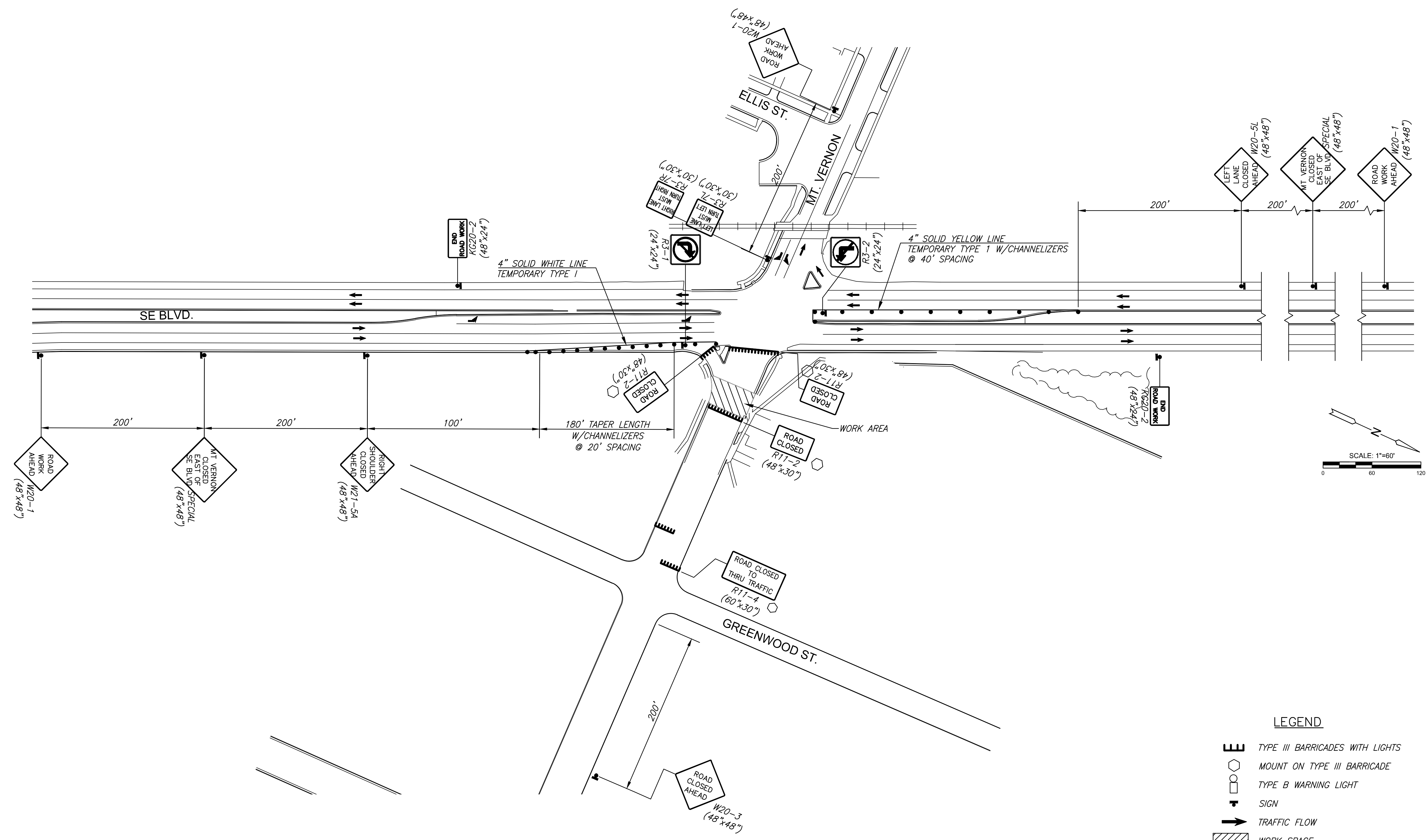
TRAFFIC CONTROL PLAN - PHASE 1
