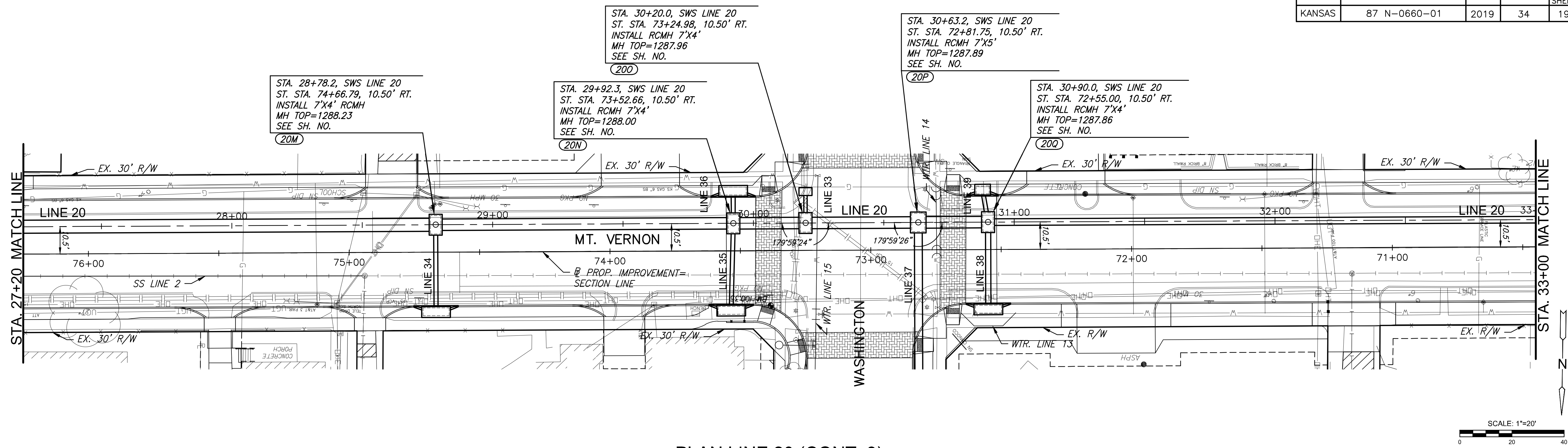
PLAN LINE 20 (CONT. 3) PROFILE LINE 20 (CONT. 3)
