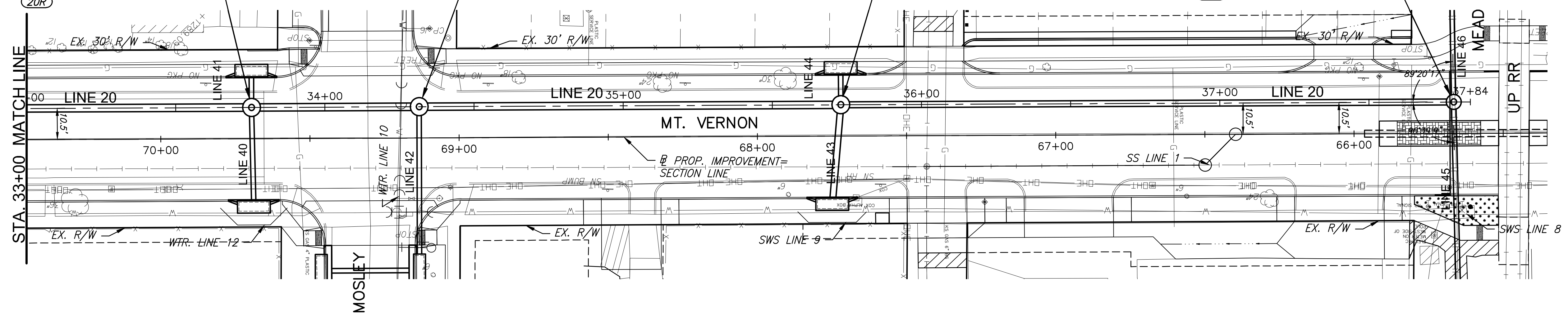
PLAN LINE 20 (CONT. 4) PROFILE LINE 20 (CONT. 4)
