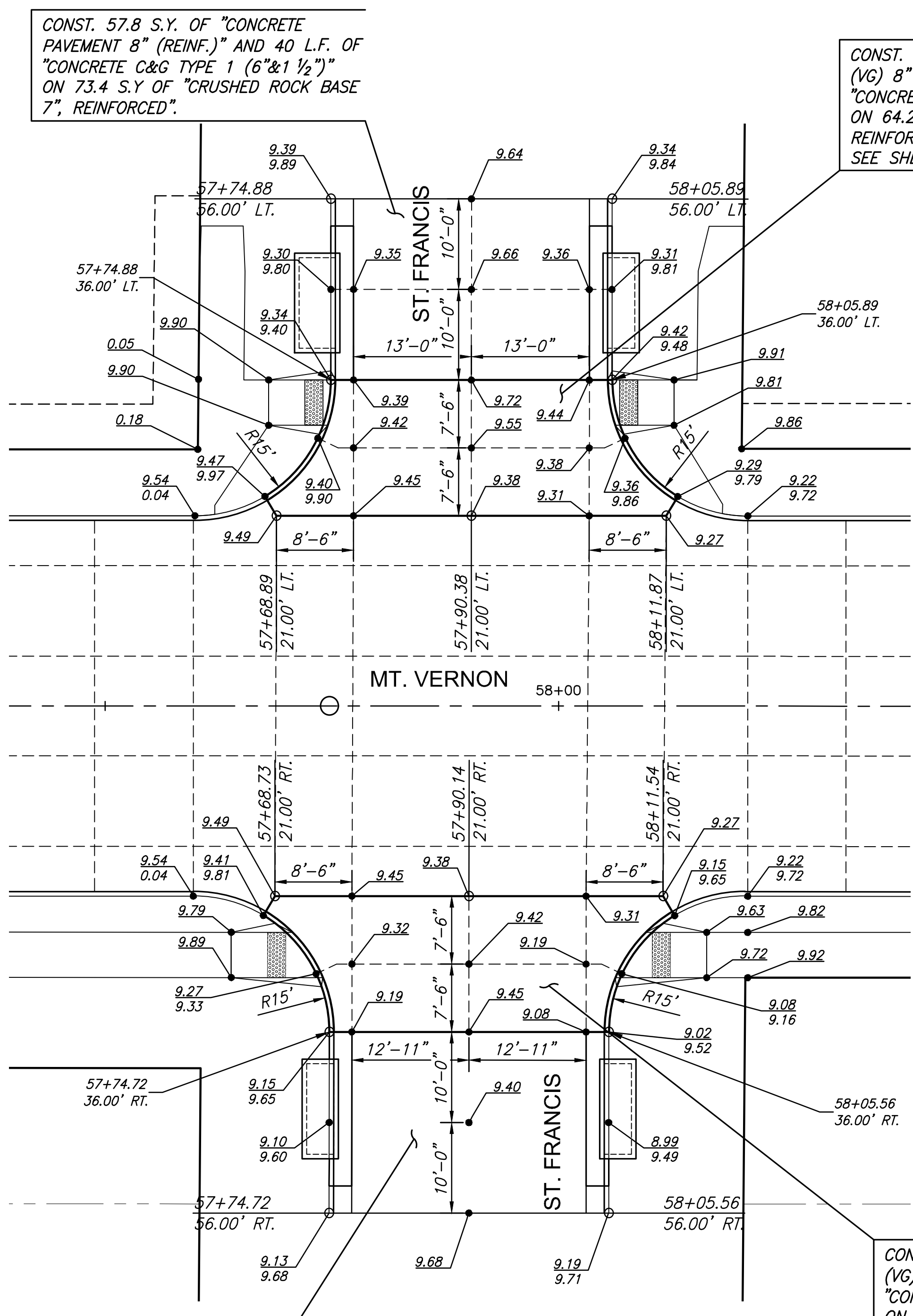
ST. FRANCIS, LT. & RT. SCALE: 1"=10'
