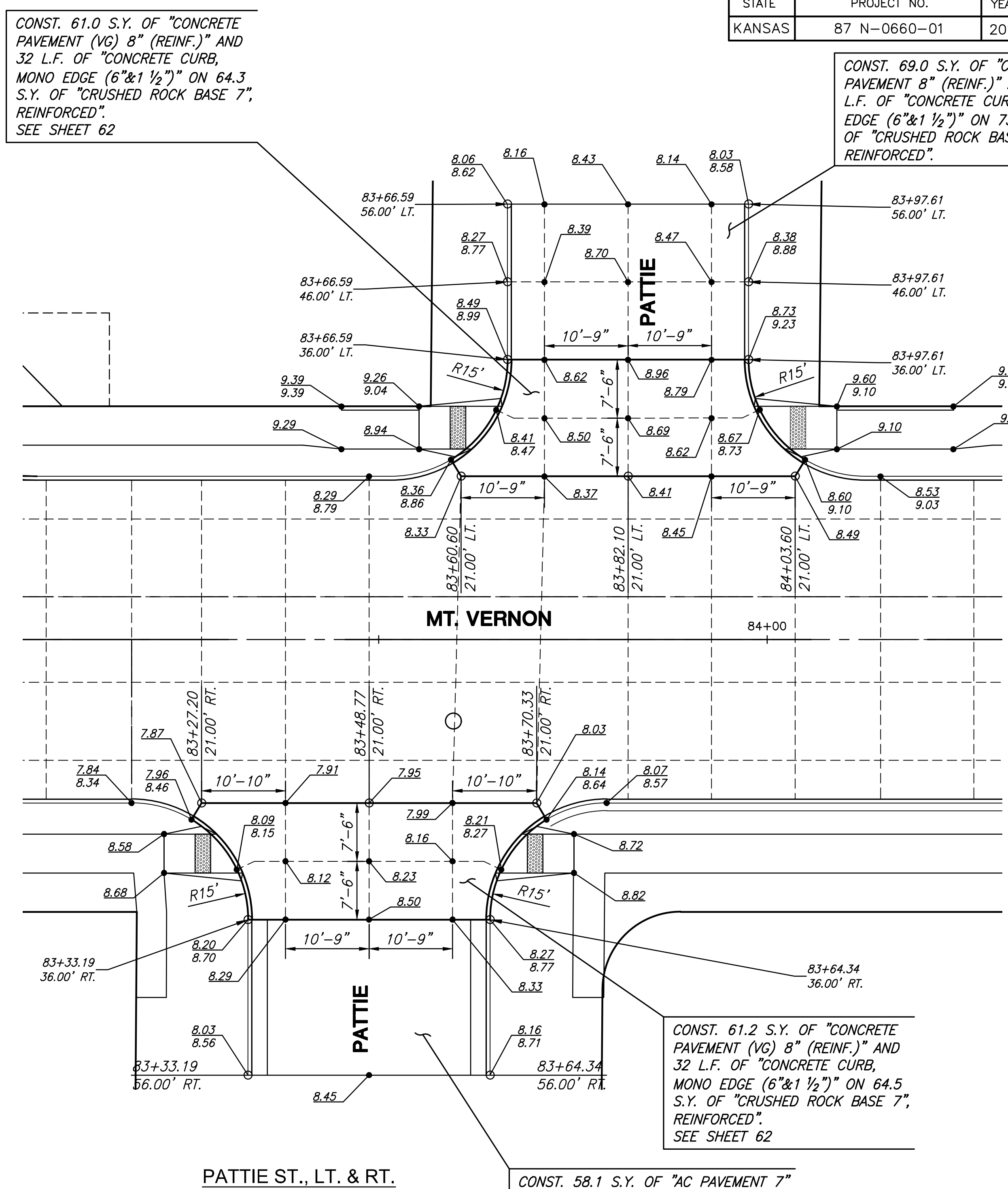
PATTIE ST., LT. & RT. SCALE: 1"=10'
