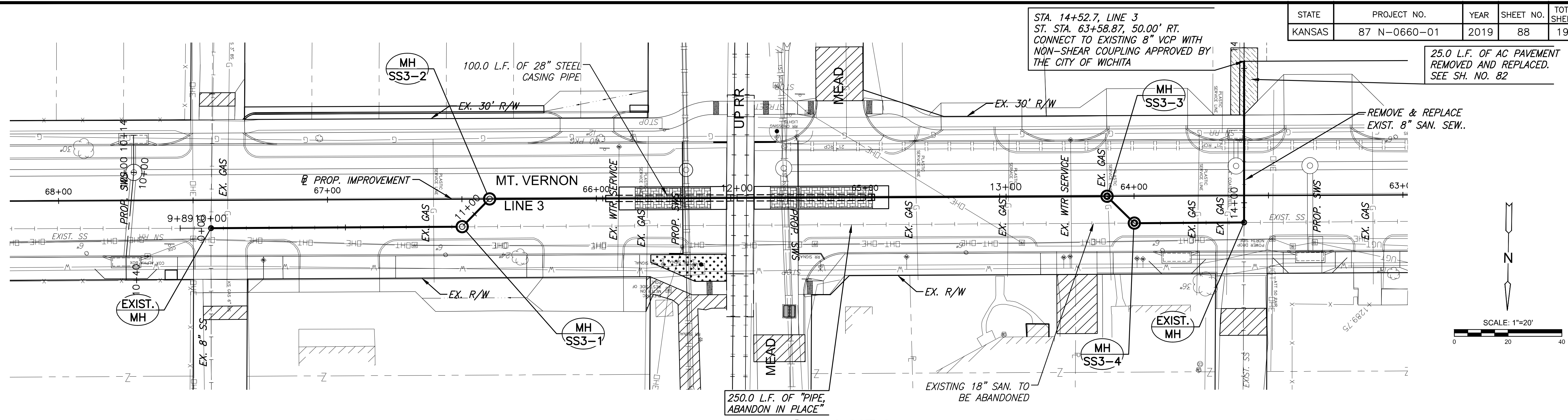
PLAN SAN LINE 3 PROFILE SAN LINE 3
