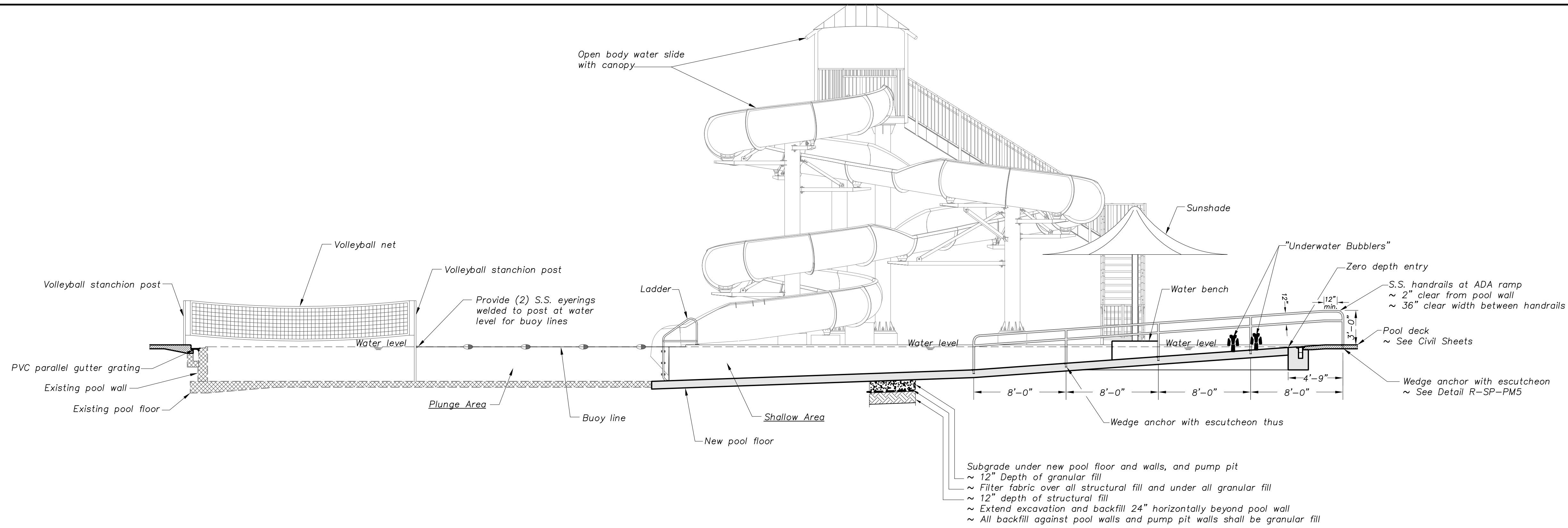
C POOL SECTION Scale: 3/16"=1'-0"
