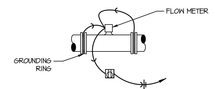
2 Flow Meter Grounding Detail Scale: None
