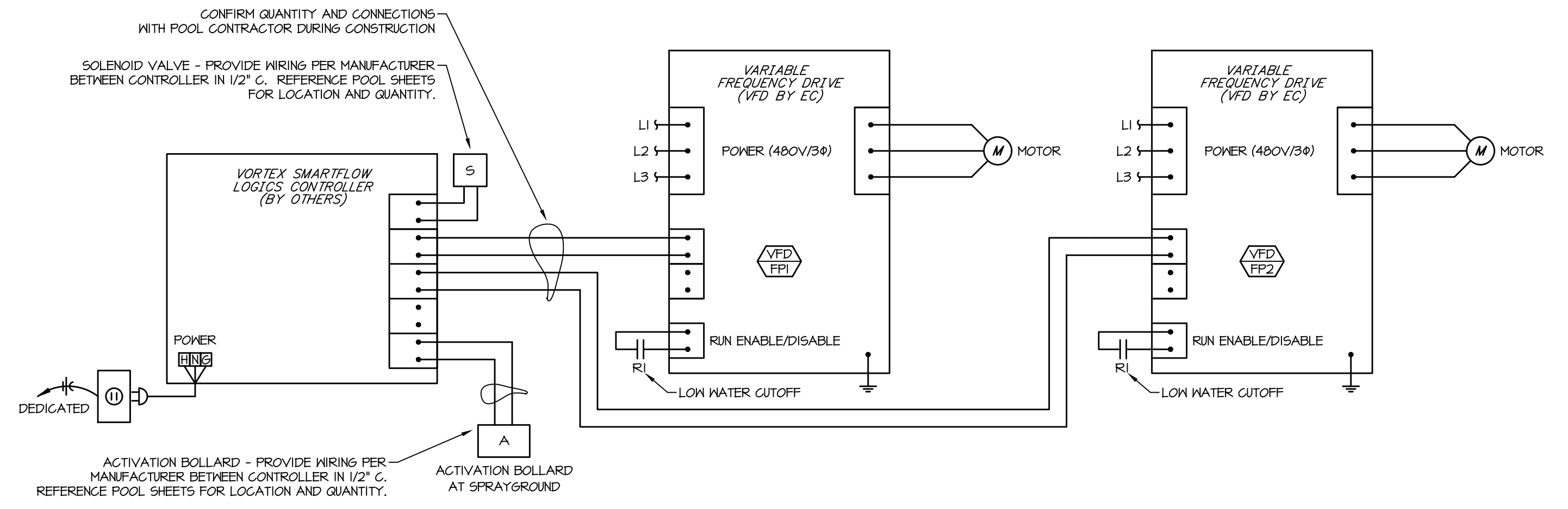
1 VFD Control Schematic (VFD-FP1, VFD-FP2) Scale: None
