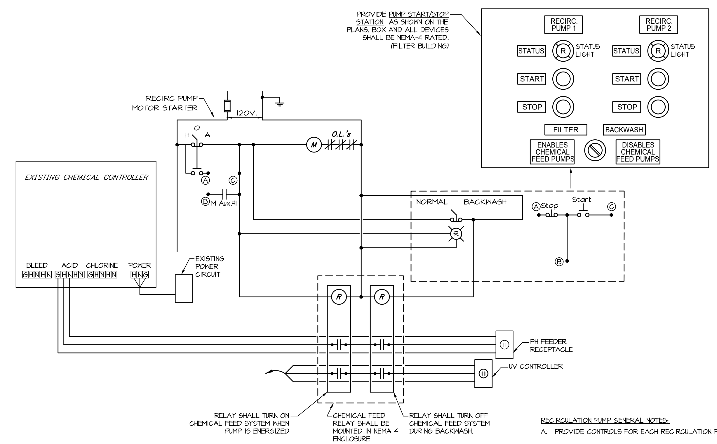
4 Recirculation Pump Control Schematic (CMS-RP1, CMS-RP2) Scale: None
