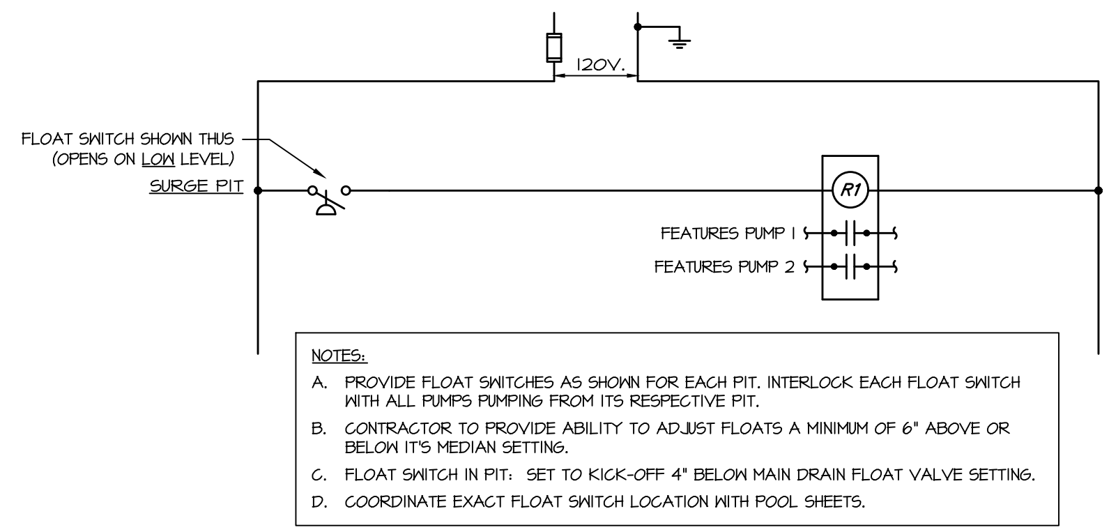
3 Motor Control Schematic Scale: None
