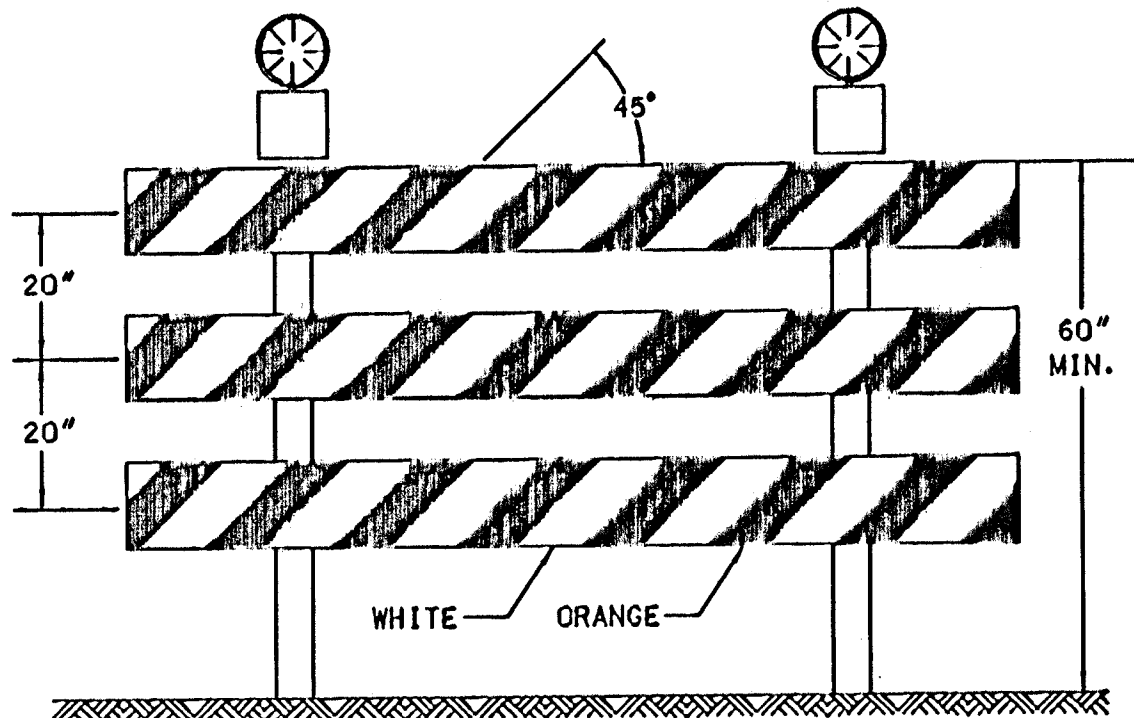
TYPE III BARRICADE WITH LIGHTS
