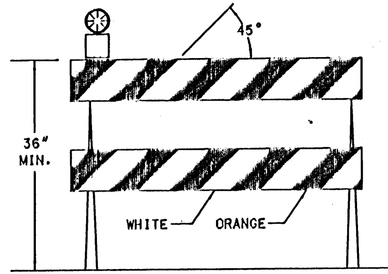
TYPE II BARRICADE WITH LIGHT
