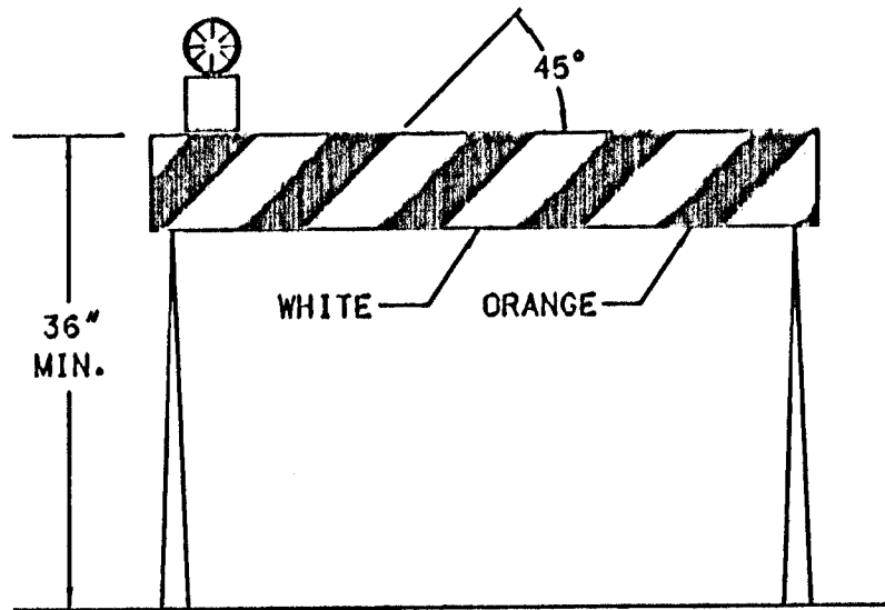
TYPE I BARRICADE WITH LIGHT
