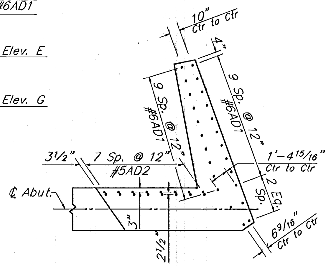
PART PLAN SHOWING AD1 & AD2 BAR SPACING
