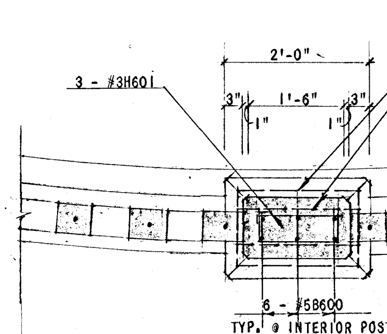
TYPICAL INTERIOR POST ON BRIDGE AND WALL AREA
