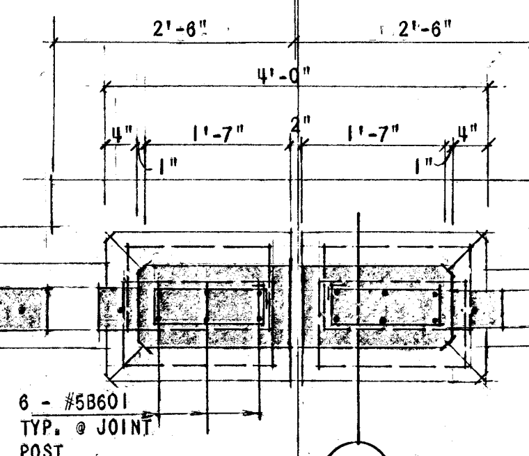
TYPICAL JOINT POST
