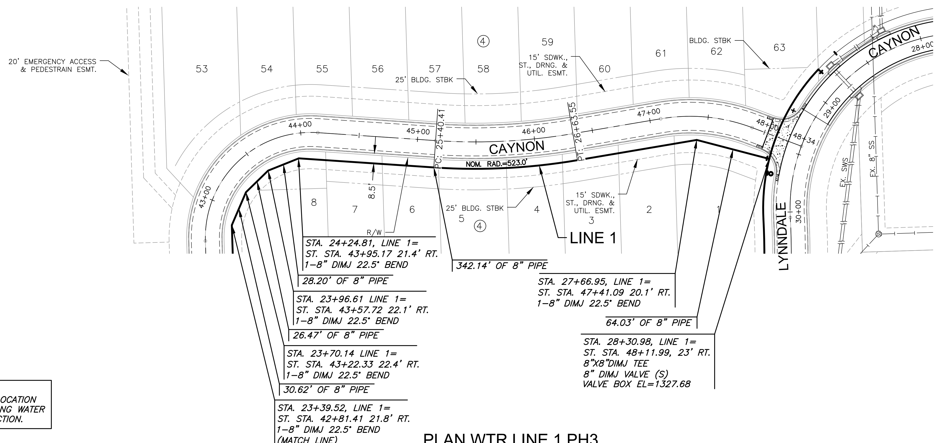
PLAN WTR LINE 1 PH3 PROFILE WTR LINE 1 PH3
