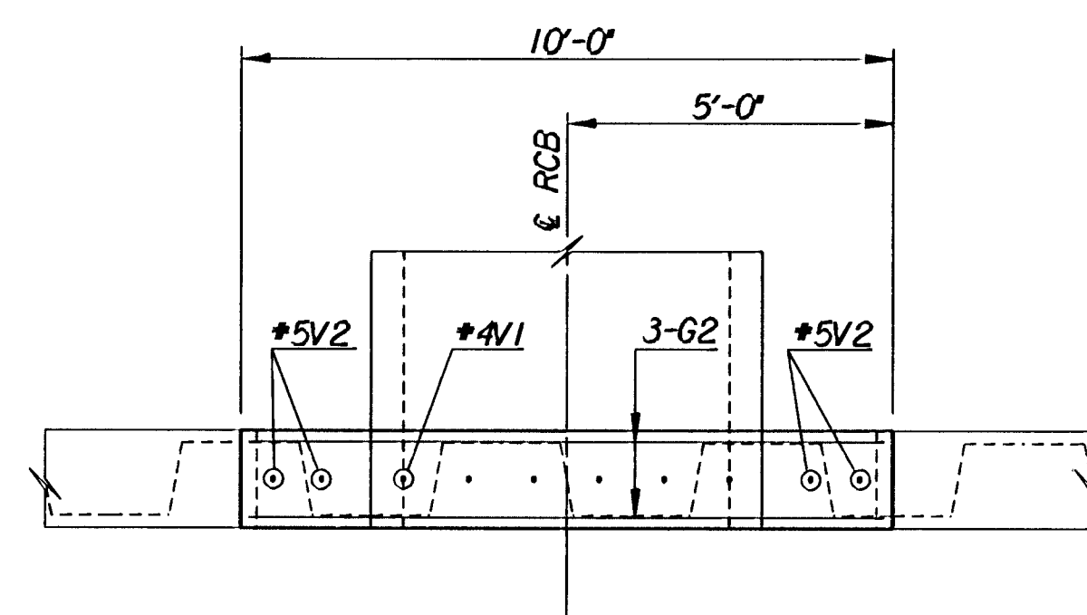
PLAN
