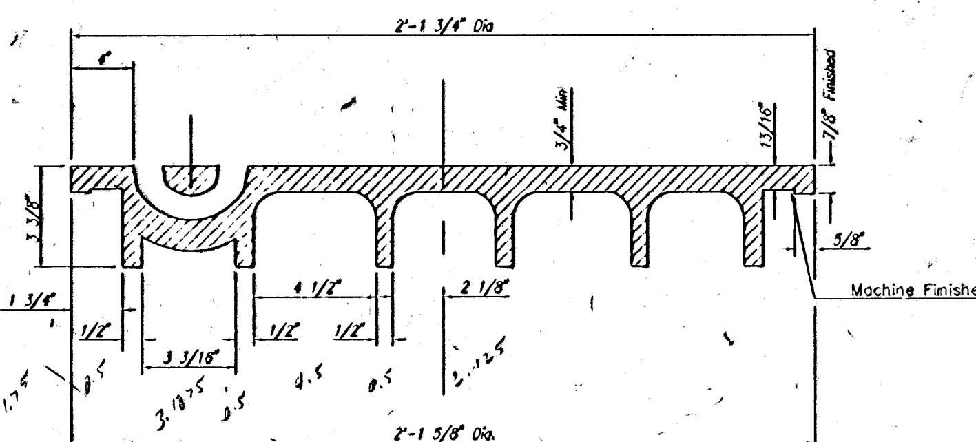
SECTION VIEW
