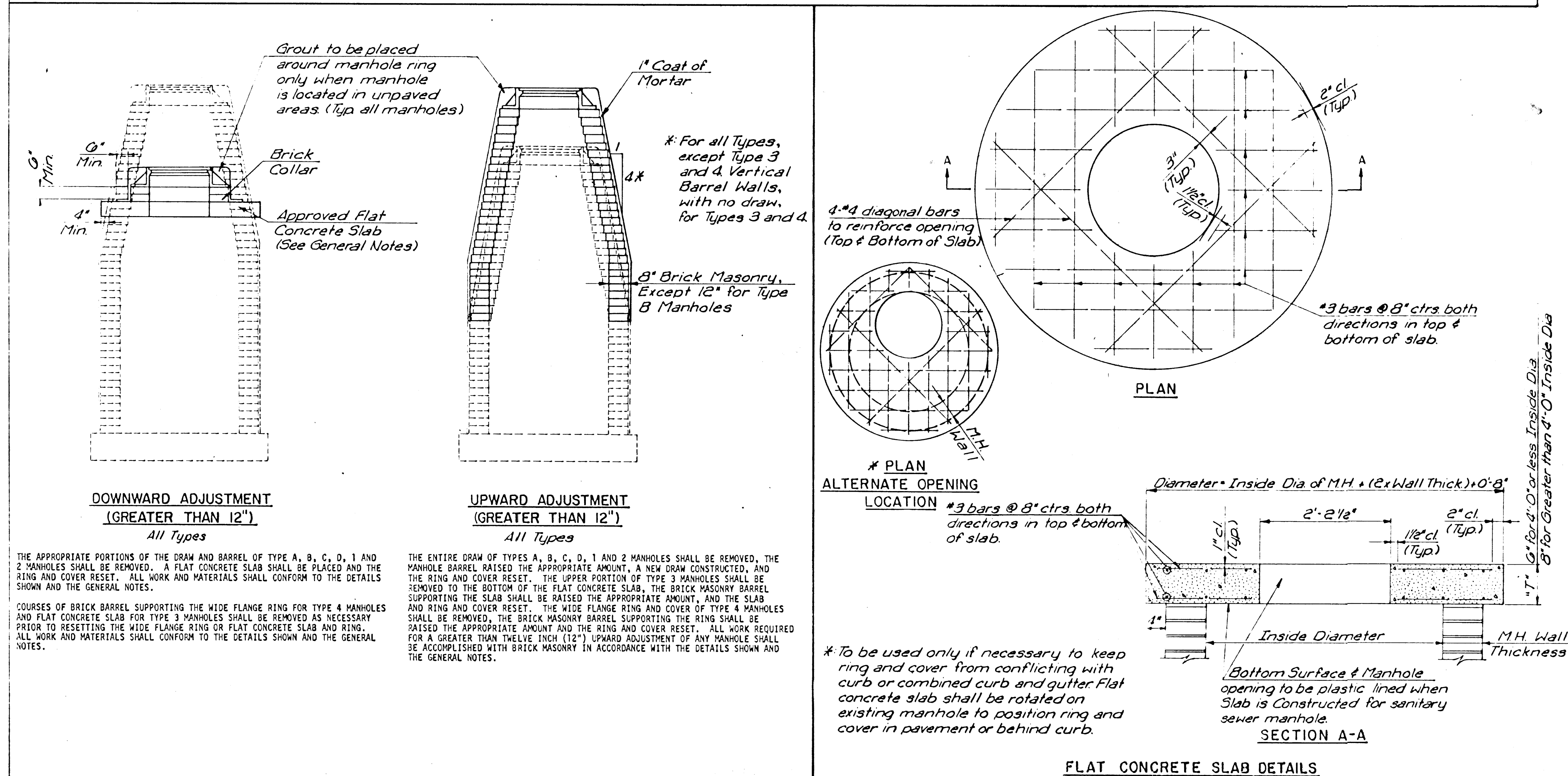
DEFINITION SKETCHES-CITY OF WICHITA STANDARD MANHOLES
