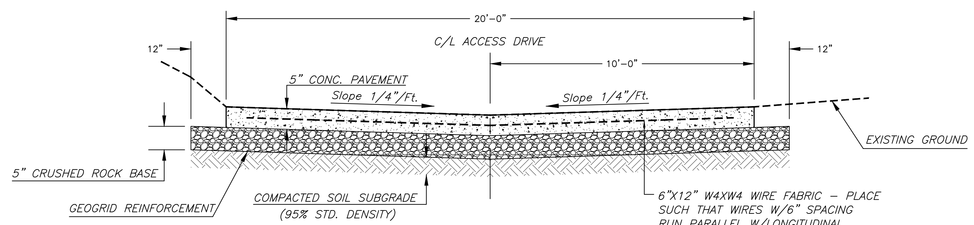
ALLEY SECTION SCALE: NOT TO SCALE
