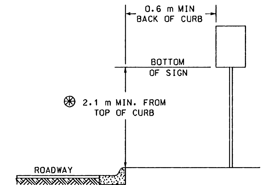
HEIGHT AND LATERAL DIMENSIONS FOR POST MOUNTED SIGNS (ALL SIGNS LEFT IN PLACE OVERNIGHT OR LONGER)
