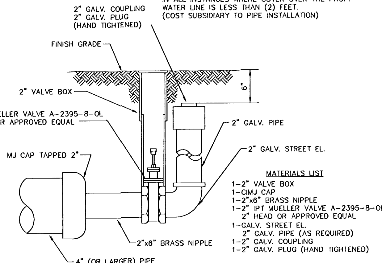
2" BLOWOFF ASSEMBLY
