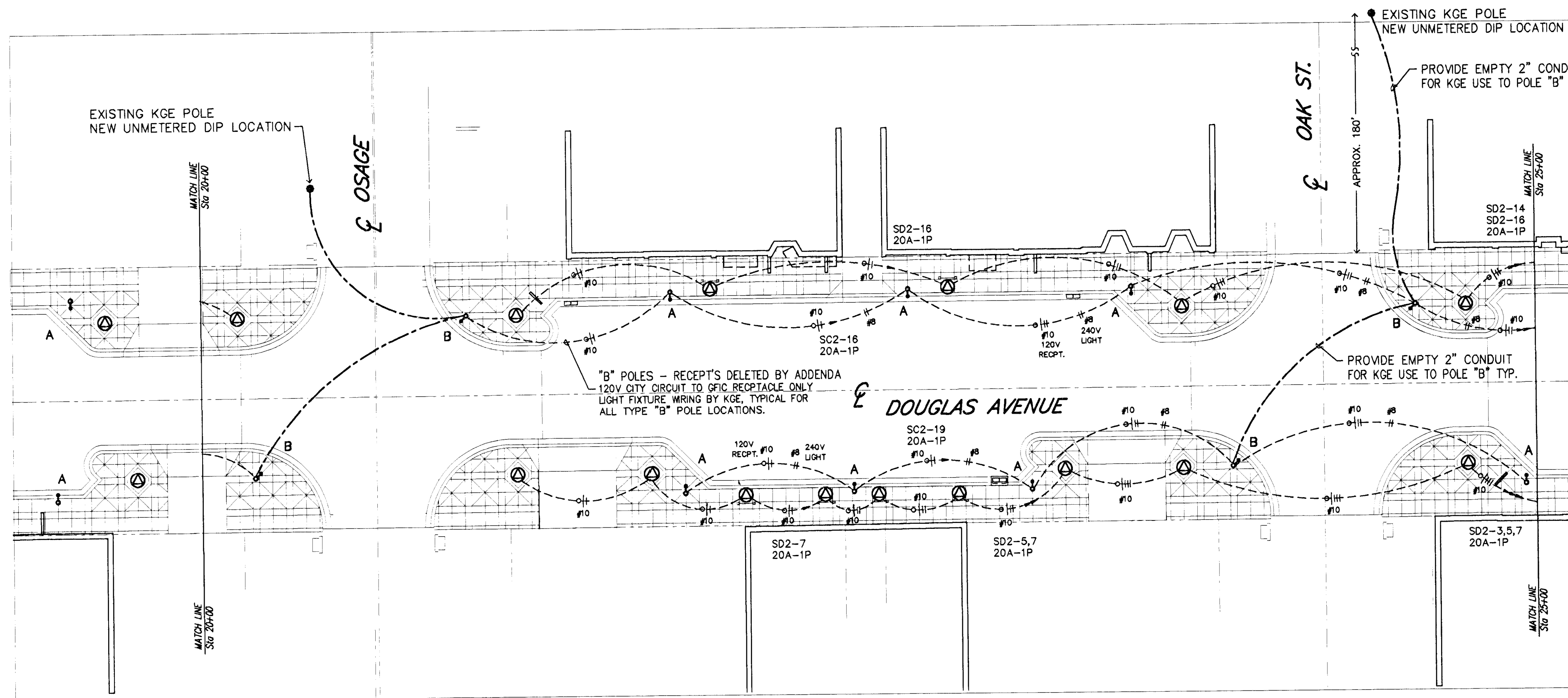
ELECTRICAL PLAN 3 1" = 30'
