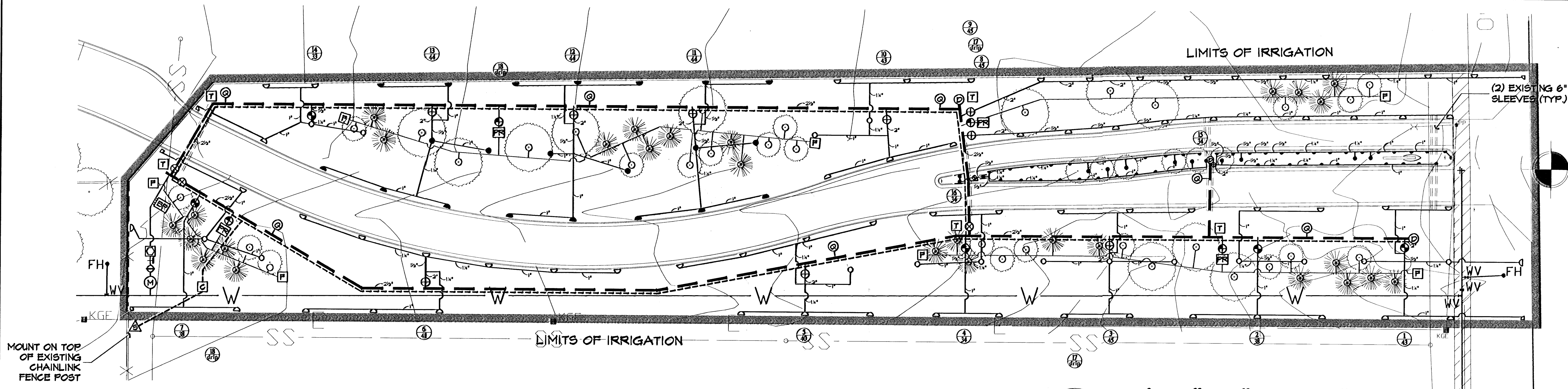
ENTRY PLAN SCALE: 1" = 30'
