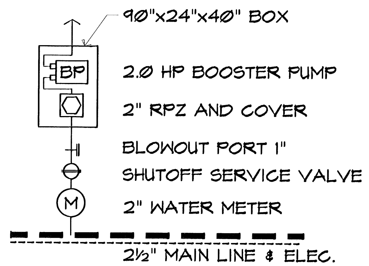
VAULT DETAIL NO SCALE
