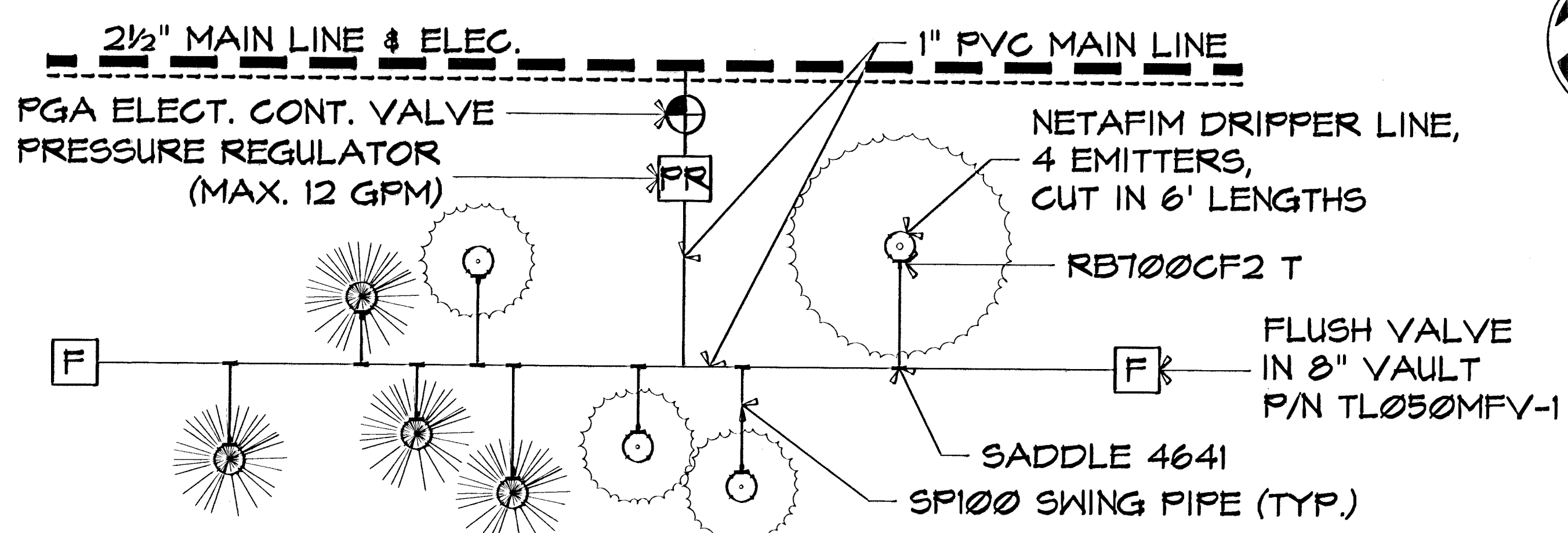
DRIP IRRIGATION DETAIL (TYP.) NO SCALE
