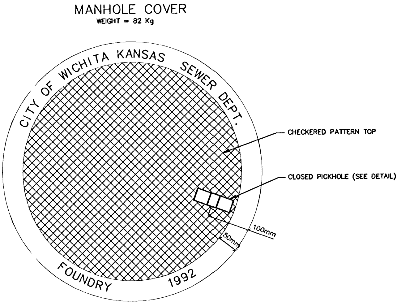
TOP VIEW
