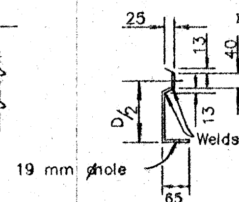
SECTION OF RECESSED FORM LEG
