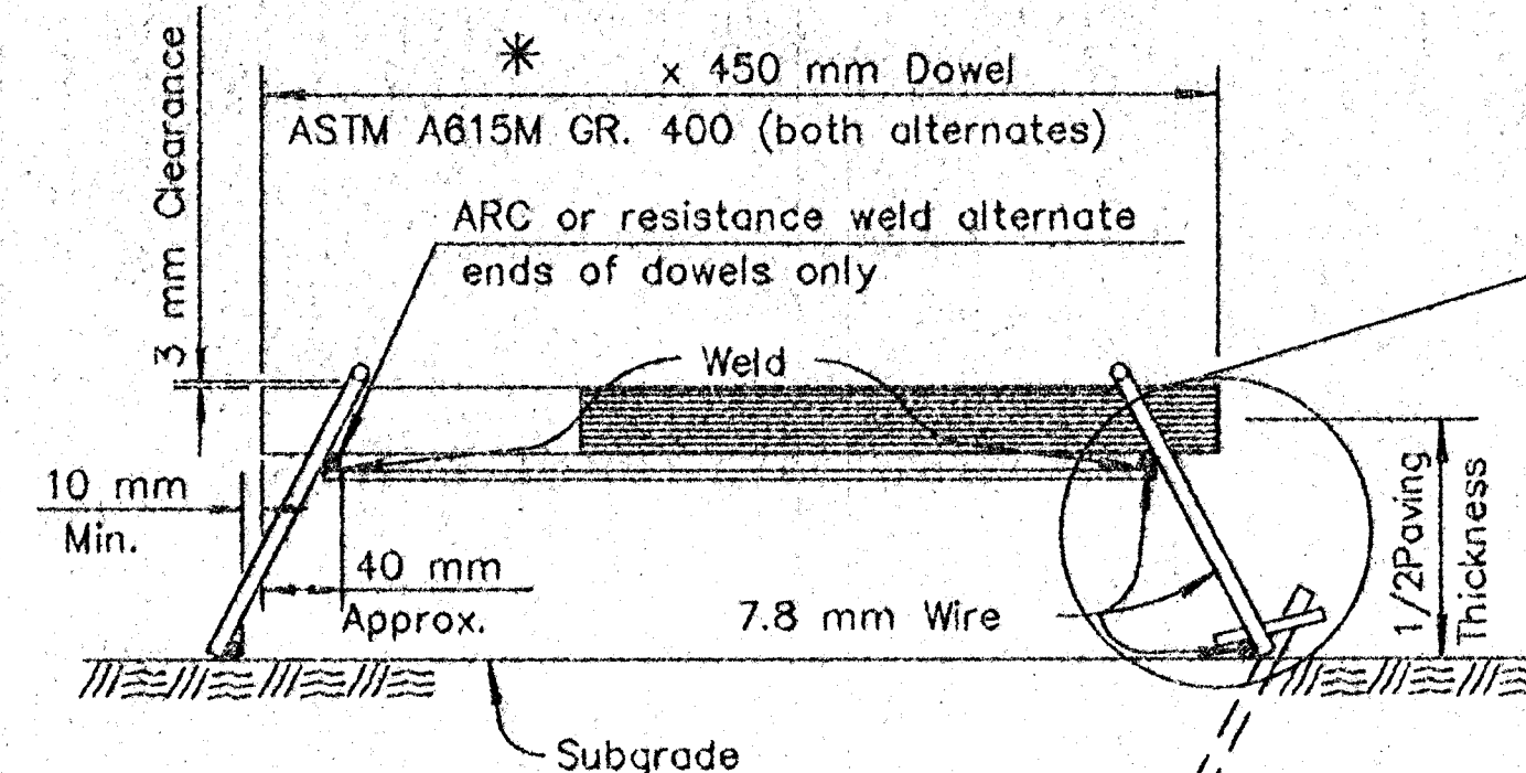
SEC. B-B
