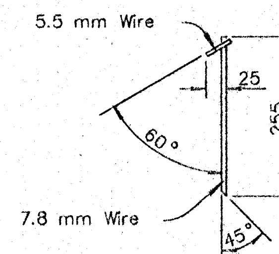
STAKE DETAIL
