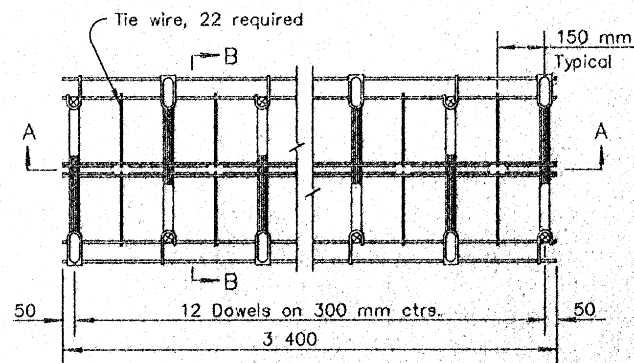
PLAN VIEW
