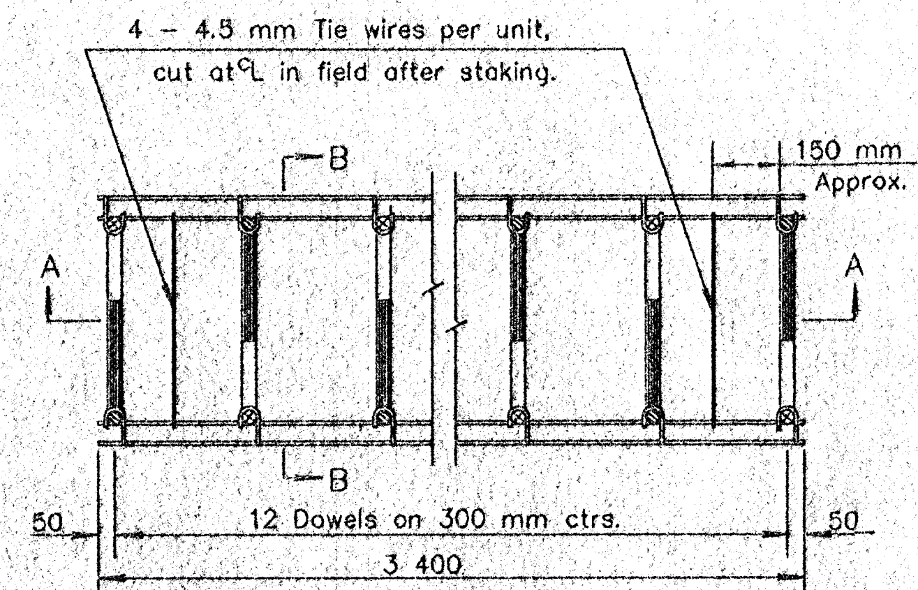
PLAN VIEW
