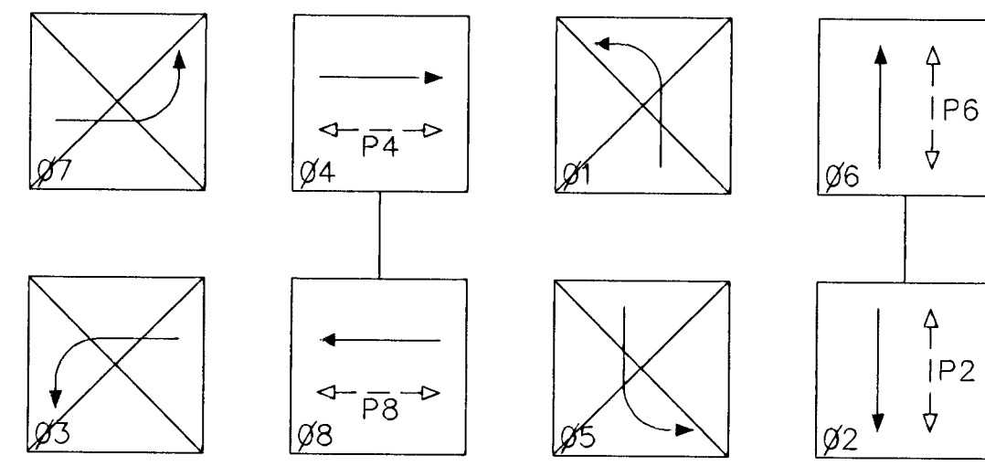
Signal Phasing
