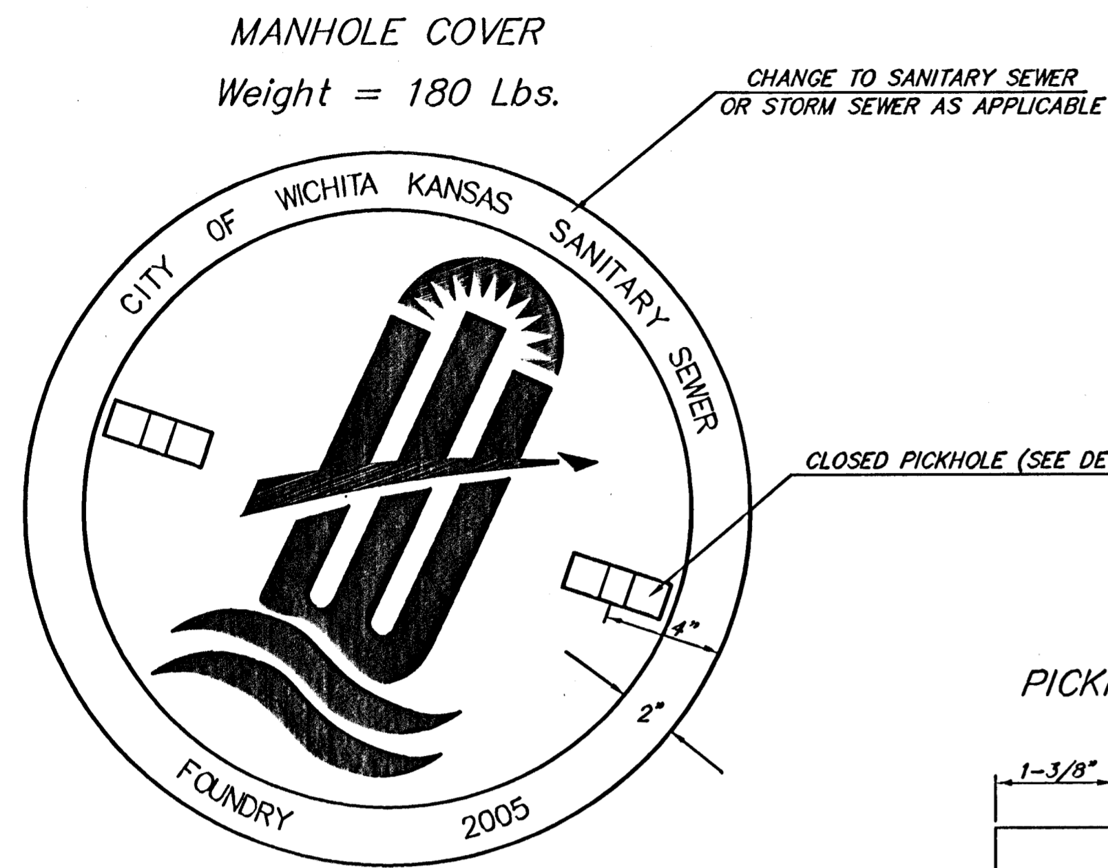
TOP VIEW
