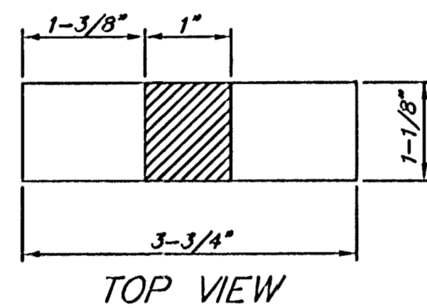
PICKHOLE DETAIL
