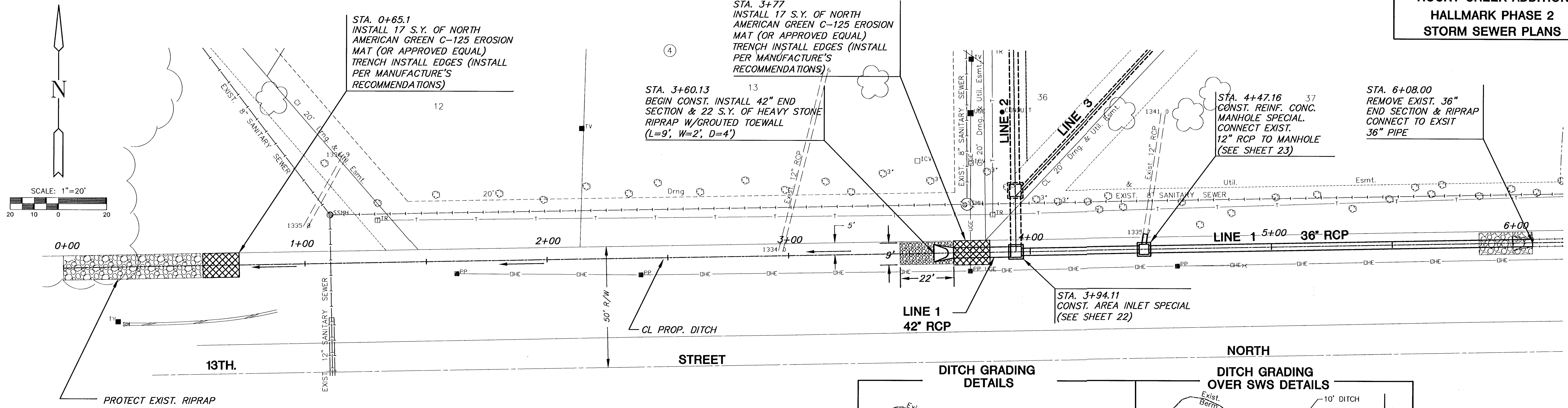
PLAN DITCH
